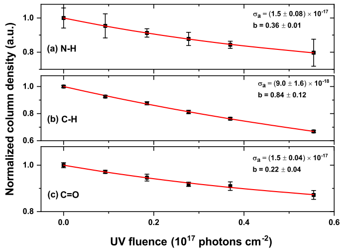
Fig. 8. Normalised column densities of the N-H (a), C-H (b) and C=O (c) of crystalline \text{NH}_2\text{CHO} on CsI at 16 K at low UV fluences (filled black squares). The normalisation factor is the corresponding initial column densities. The best fit to the data (red solid lines) is also shown. The estimated amorphisation rate ( \sigma_a ) and the asymptotic transformation ( b ) for \text{NH}_2\text{CHO} are also provided.
