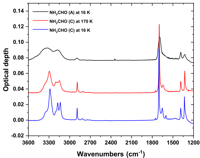
Fig. 4. A comparison of mid-IR spectra for a 23.4 ML \text{NH}_2\text{CHO} film deposited on a CsI substrate under different temperature conditions. The top curve in black represents the spectrum at 16 K immediately after deposition. The middle curve in red corresponds to the spectrum after heating the sample to 170 K, and the bottom curve in blue represents the spectrum upon cooling back to 16 K. The ice upon warming up crystallizes and shows sharp features which are irreversible even after cooling back to 16 K. For clarity in visualization, the black, red, and blue curves have been offset along the vertical axis by 0.04, 0.04, and -0.04 units, respectively. It is worth noting that the crystalline phase of ice is indicated as 'C' in the spectra.
