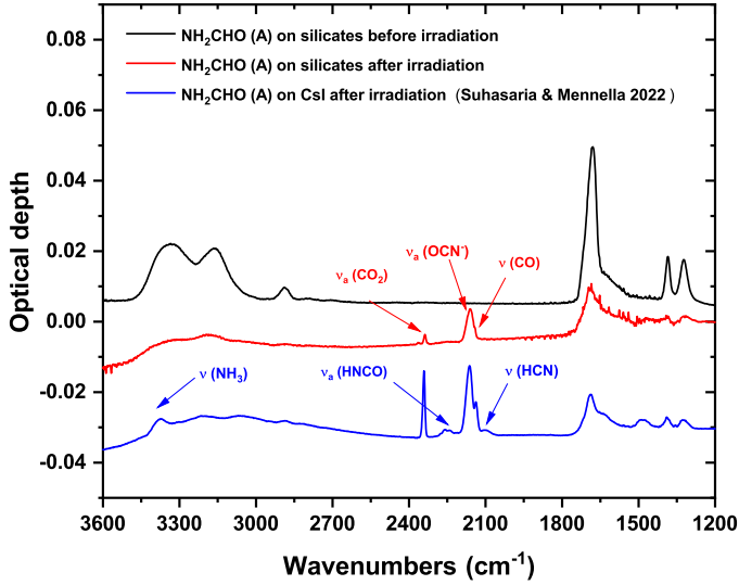
Fig. 1. The mid-IR spectrum represents a 29.5 monolayer (ML) amorphous \text{NH}_2\text{CHO} film at 16 K deposited on amorphous silicates, indicated by the black line. After irradiation with a UV fluence of 3.7 \times 10^{18} photons \text{cm}^{-2} (red line), changes in the spectrum are observed, highlighted by arrows. The symbols \nu indicate stretching vibrations, and the subindex a signifies antisymmetric mode. For comparison, we also present the spectrum of a 29.5 ML thick amorphous \text{NH}_2\text{CHO} film on a blank CsI substrate following the same UV fluence as above, (blue line; Suhasaria & Mennella (2022)). The red and blue curves have been vertically shifted by 0.008 and -0.03, respectively, for clarity. Please note that the amorphous phase of ice is denoted by 'A'.
