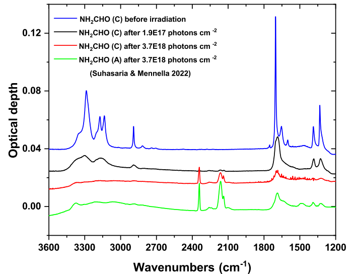
Fig. 5. Mid-IR spectrum of a 23.4 ML crystalline \text{NH}_2\text{CHO} film on CsI at 16 K (blue line) and after irradiation with UV fluences of 1.9 \times 10^{17} photons \text{cm}^{-2} (black line) and 3.7 \times 10^{18} photons \text{cm}^{-2} (red line), respectively. The crystalline ice is rapidly transformed to the amorphous form after just the first irradiation step as seen from the black line. The spectrum of a 29.5 ML amorphous \text{NH}_2\text{CHO} film on a blank CsI substrate after a fluence of 3.7 \times 10^{18} photons \text{cm}^{-2} (green line) is also shown for comparison (Suhasaria & Mennella 2022). The black curve is offset in ordinate by -0.01 for the sake of clarity.
