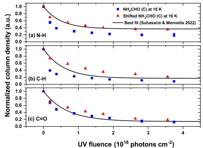
Fig. 6. Normalised column densities of the N-H (a), C-H (b) and C=O (c) (filled blue circles) of crystalline \text{NH}_2\text{CHO} on CsI at 16 K with increasing UV photon fluence. The normalisation factor is the corresponding initial column densities. For the sake of simplicity, the evolution is compared with the best fit to the data (black solid line) presented for amorphous \text{NH}_2\text{CHO} on CsI at 12 K (Suhasaria & Mennella 2022). The two results tend to match if the first data point of the crystalline ice is subtracted and re-normalized (red triangles).
