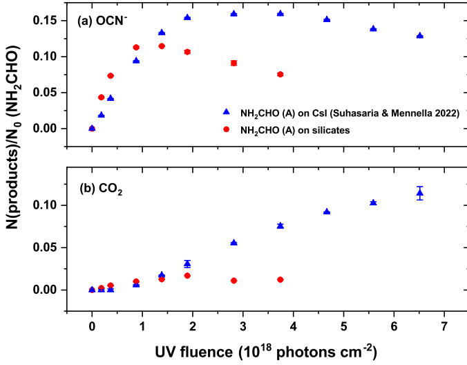
Fig. 3. Evolution in normalised column densities of \text{OCN}^- (a) and \text{CO}_2 (b), represented by red filled circles, as a function of increasing UV photon fluence on amorphous \text{NH}_2\text{CHO} adsorbed on amorphous silicates. The normalisation factor is the column density of \text{NH}_2\text{CHO} before UV irradiation. The infrared absorption areas are determined through Gaussian fitting, with error bars representing one standard deviation. In cases where the error bars are not visible, they are within the size of the data points. These results are compared with the evolution data of \text{OCN}^- and \text{CO}_2 , indicated by blue filled triangles, following UV irradiation of amorphous formamide on a clean CsI substrate (Suhasaria & Mennella 2022).
