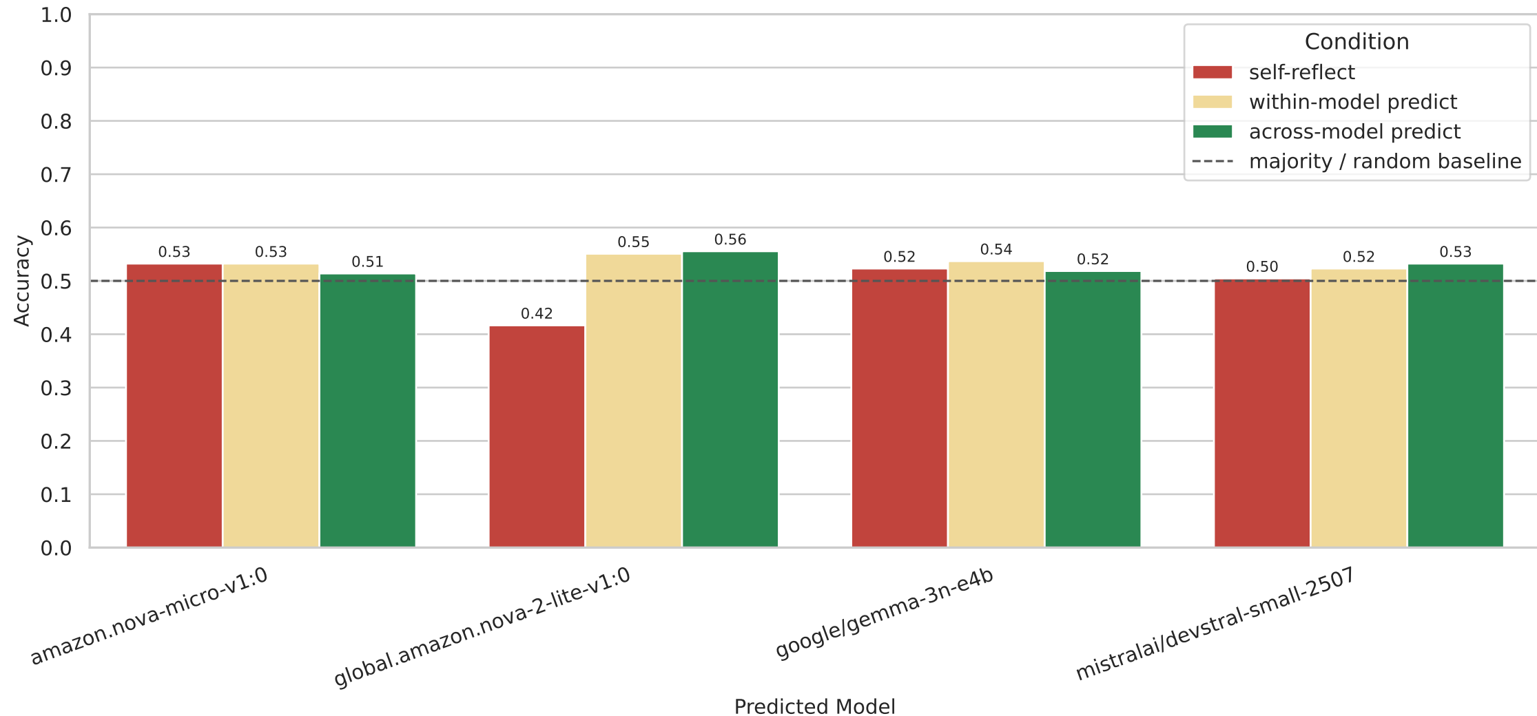
Study 2: Accuracy by condition
