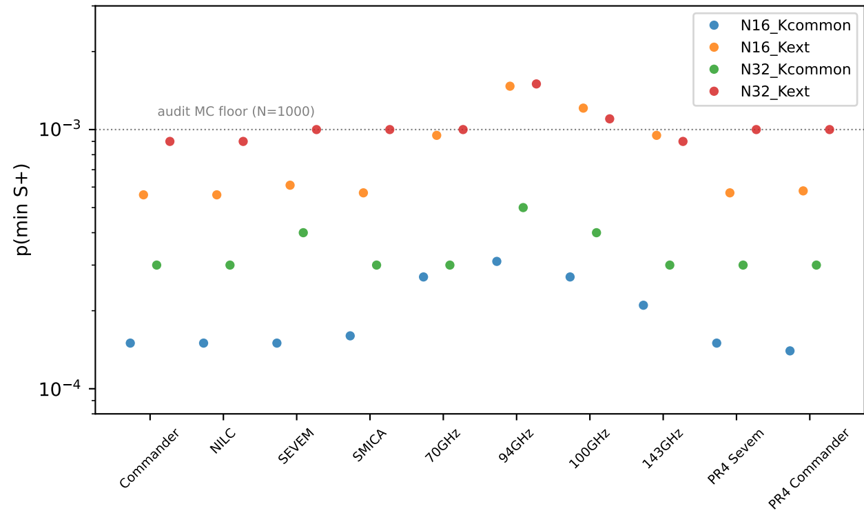
Plane-excised mirror anti-symmetry measured below the floor
