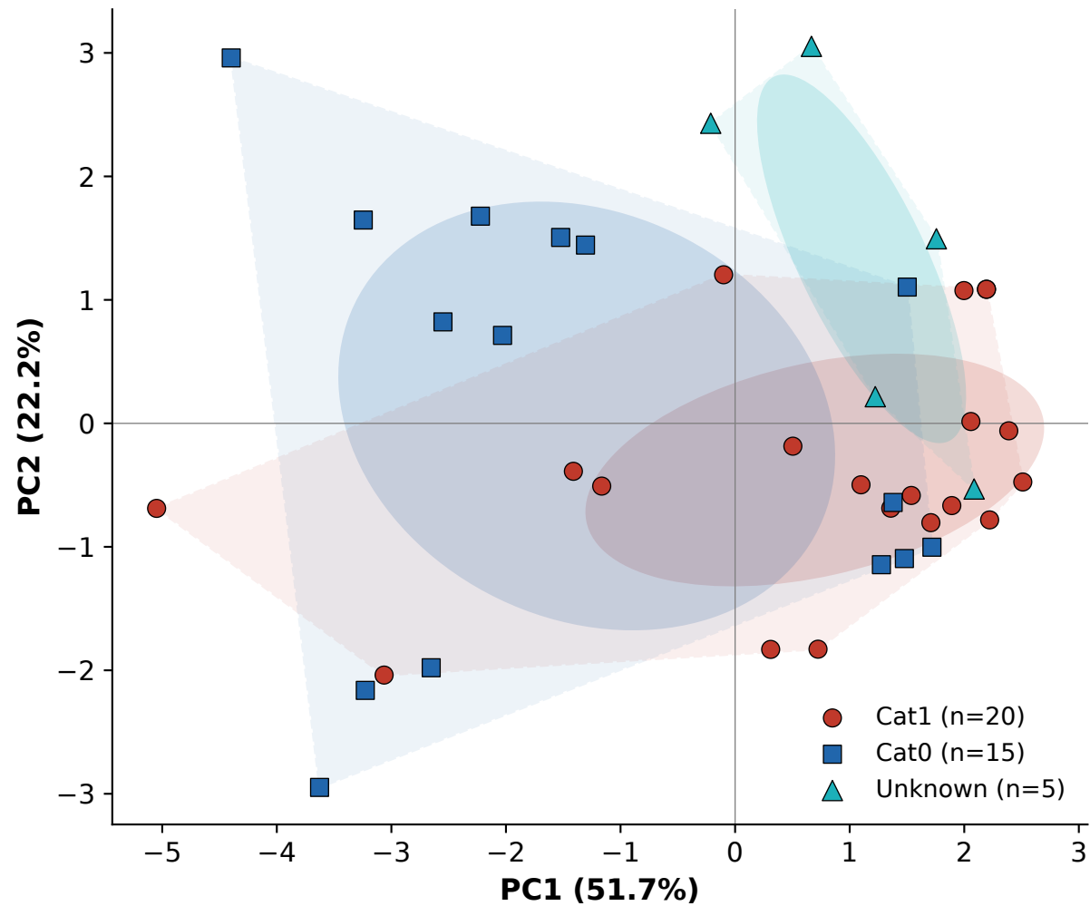
a 10 original descriptors
