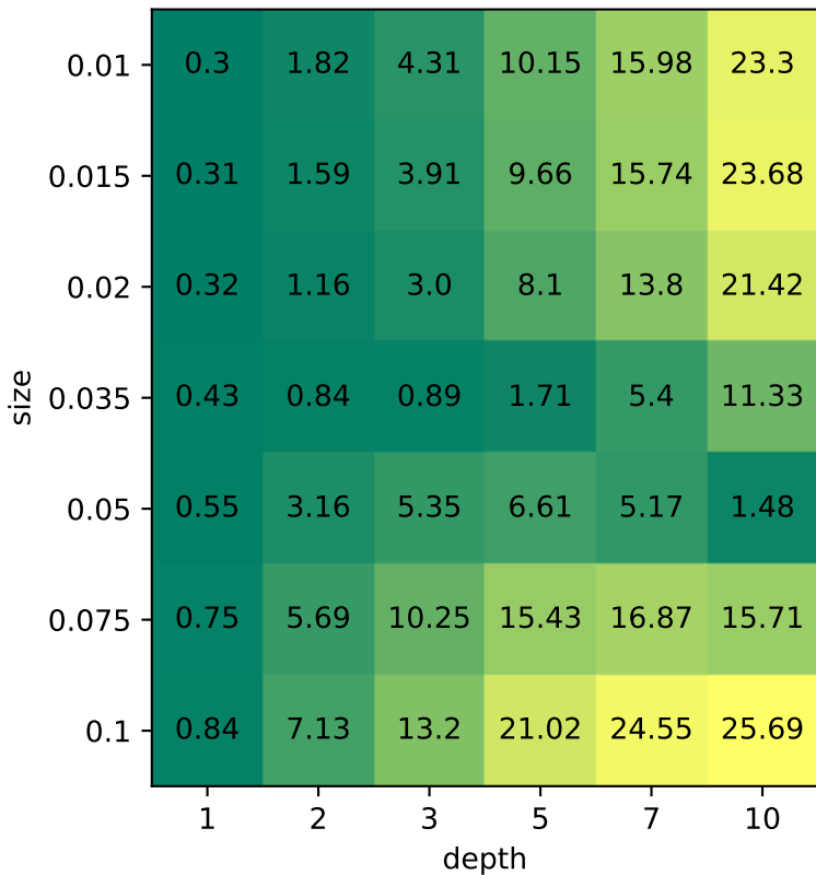
Mean Absolute Error
