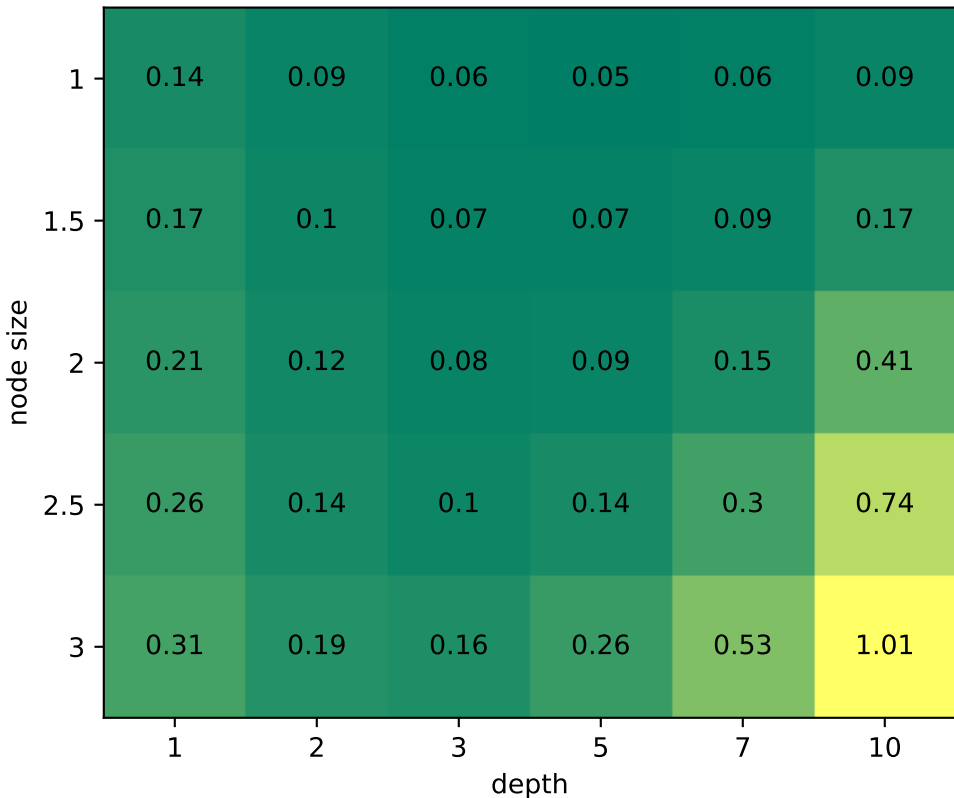
Mean Positive Error
