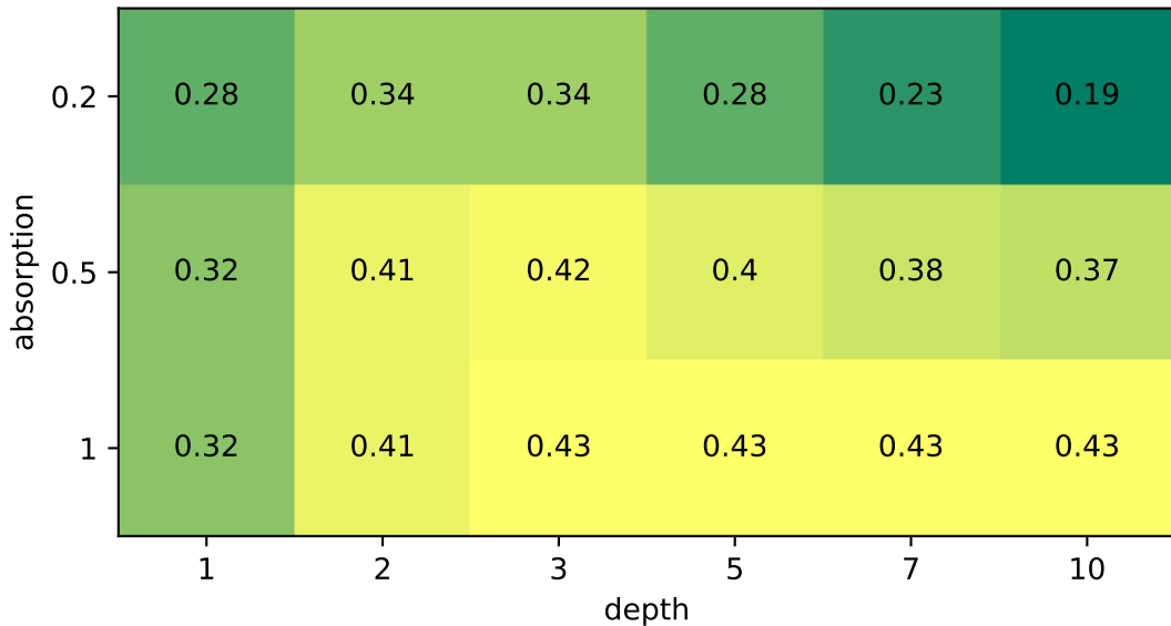
Mean Negative Error
