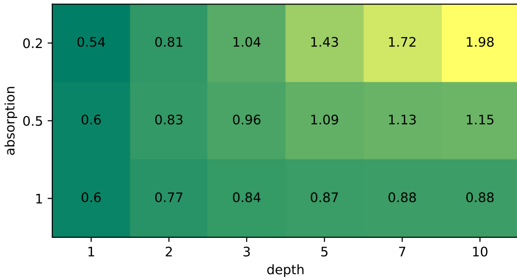
Mean Absolute Error
