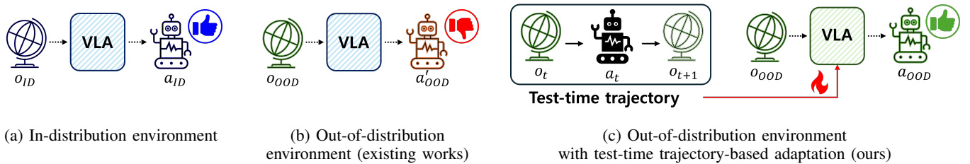
Fig. 2: Comparison of VLAs under in-distribution and out-of-distribution. Blue denotes the in-distribution training domain, green indicates the out-of-distribution domain at test time, and orange represents inconsistent action outputs induced by distribution shifts. (a) In an in-distribution setting, observations align with the training distribution of the VLA, resulting in consistent visual–action representations. (b) Under an out-of-distribution environment, visually shifted observations lead to mismatches between visual inputs and action representations in the pre-trained VLA. (c) Our method effectively adapts the pre-trained VLA using a test-time trajectory in the shifted environment, mitigating visual–action inconsistencies.
