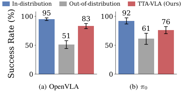
Fig. 7: Real-world success rates under in-distribution and out-of-distribution settings. For each backbone, results are averaged over the evaluated real-world settings, and error bars denote standard errors.
