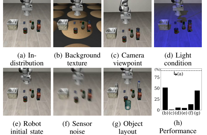
Fig. 1: Examples of various visual perturbation types in LIBERO-Plus [10], along with their performance on Open-VLA [3]. Original performance without visual perturbation, exemplified by (a), is plotted as a dashed line in (h).
