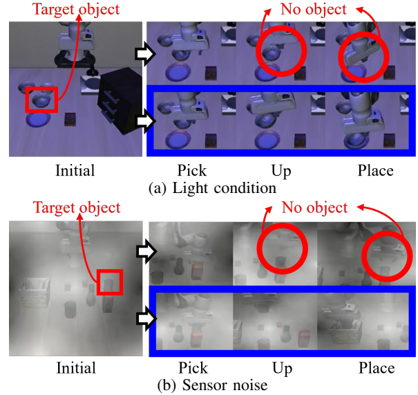
Fig. 6: Visualizations of rollouts with the original policy (top row) and TTA-VLA (bottom row) on LIBERO-Plus under (a) light condition and (b) sensor noise perturbations. Key failure scenes are highlighted with red circles, while successful executions are highlighted with blue boxes.
