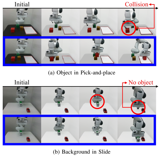
Fig. 8: Real-world rollouts between the original policy (first row) and our method (second row). Key failure scenes are highlighted with red circles, while successful executions are highlighted with blue boxes.
