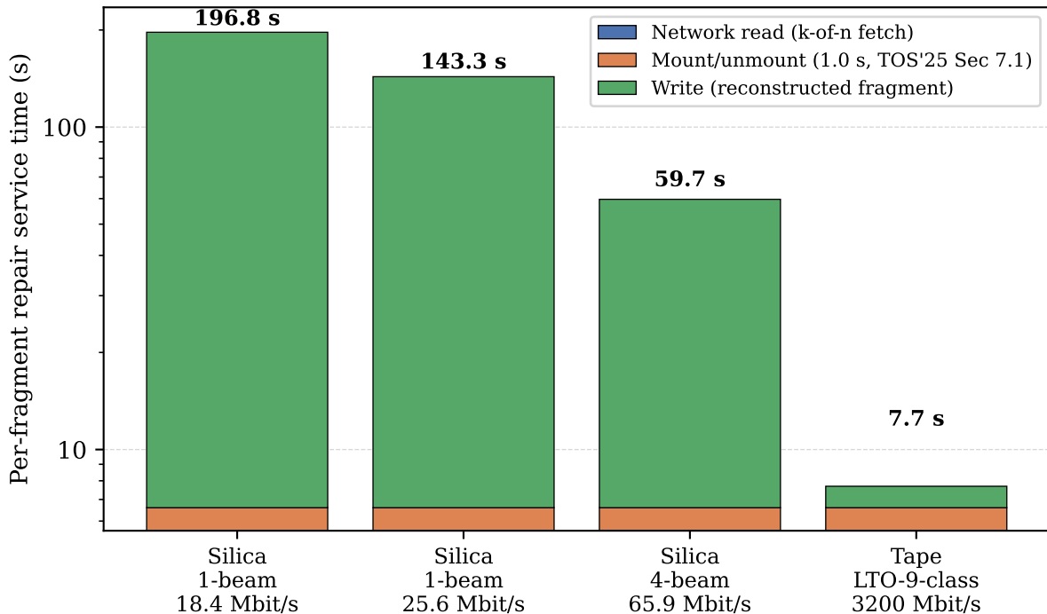
Repair service-time decomposition: mount vs. write dominance ( k=16, n=19 erasure-coded fragment, single repair job)
