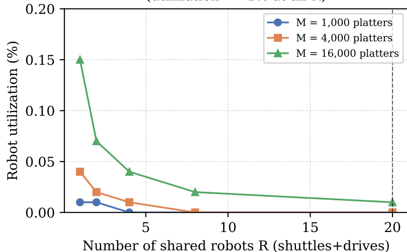
(b) Robots are never the bottleneck (utilization \ll 1% at all R)
