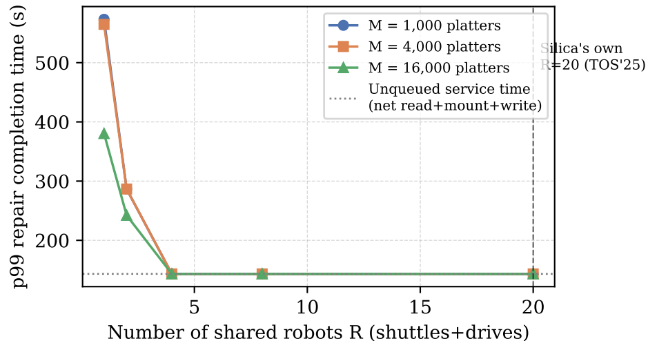
(a) Queueing delay collapses by R=4
