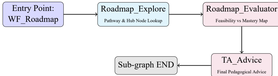
Figure 4.7: Roadmap sub-graph.
