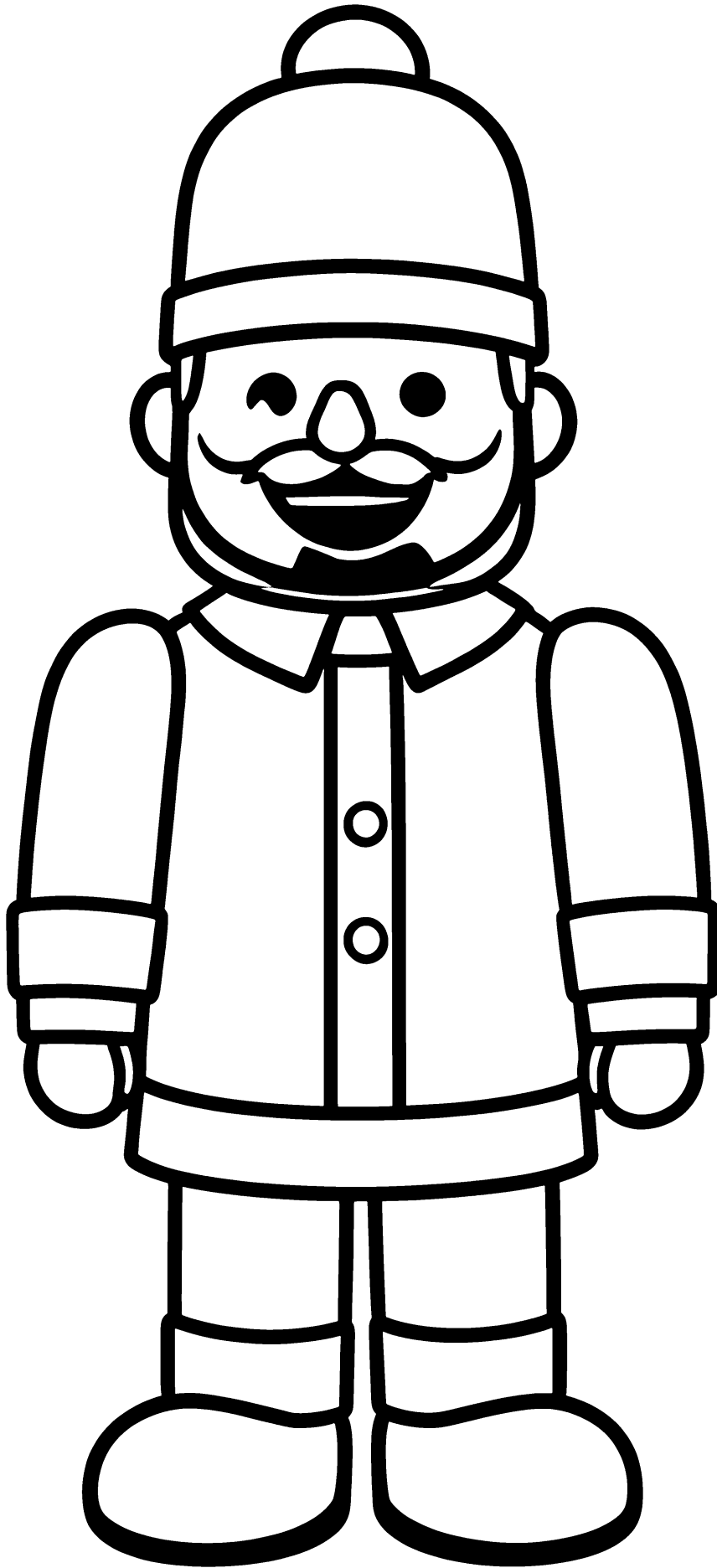
Toy Soldier
