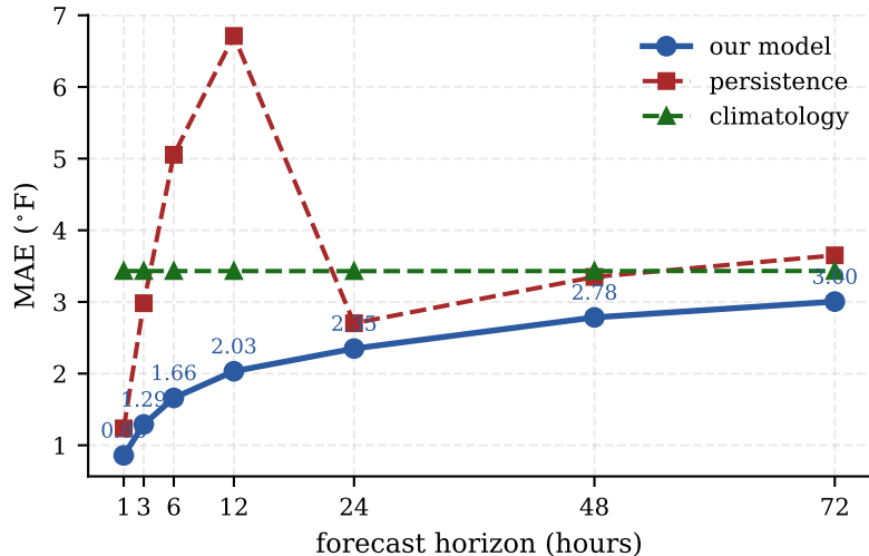
Test-set MAE vs baselines
