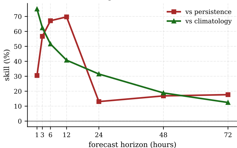
Skill scores (positive = beat baseline)
