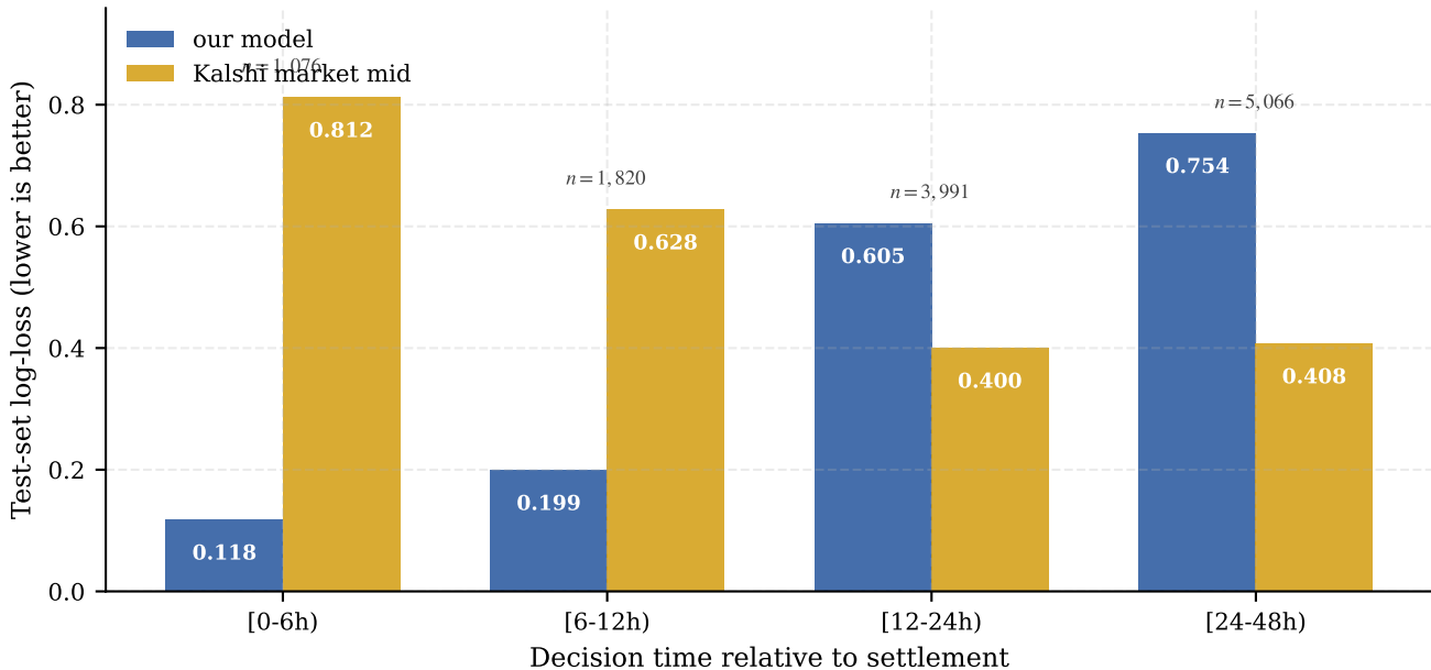
Probabilistic skill: model vs Kalshi market by horizon to settlement
