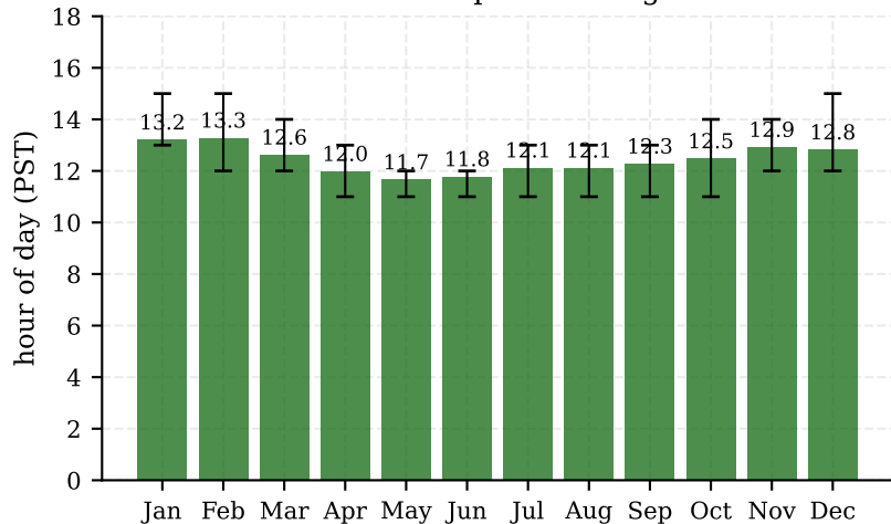
Mean hour of day SFO daily HIGH occurs (PST) with interquartile range
