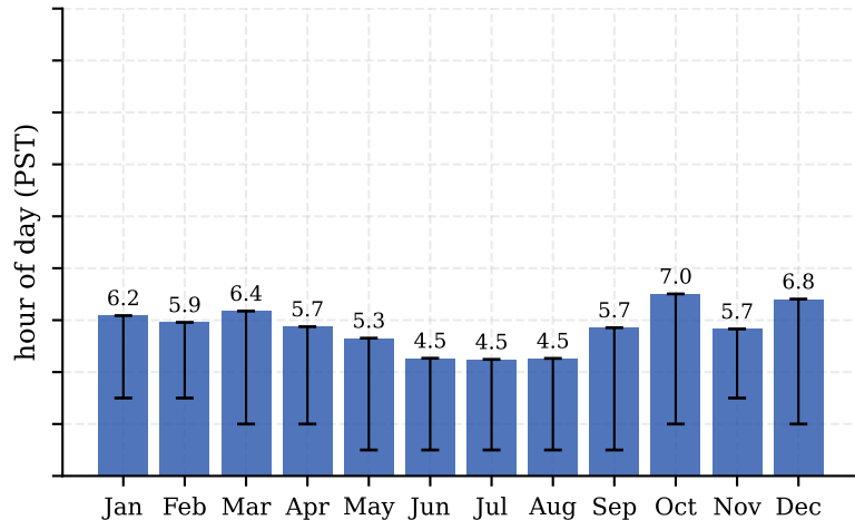
Mean hour of day SFO daily LOW occurs (PST) with interquartile range
