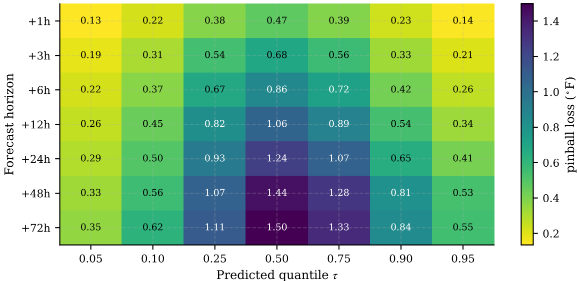
Validation pinball loss PL_\tau (lower is better, units ^{\circ}\text{F} )
