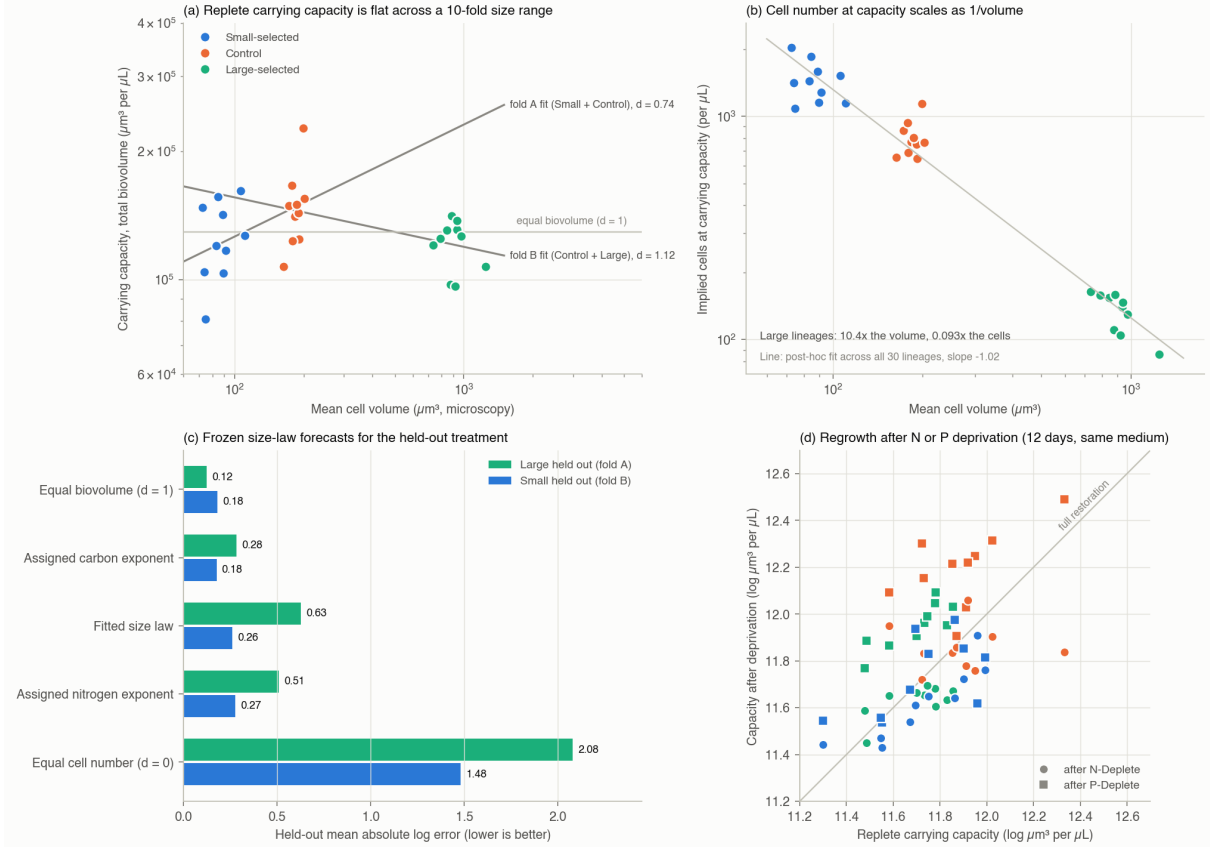
Figure 4. Size-selected Dunaliella lineages regrown in one shared medium, from the data of Malerba et al. (2018). (a) Replete carrying capacity in total biovolume against mean cell volume, with the two cross-fitted size laws and the equal-biovolume law. (b) Implied cell number at capacity. (c) Held-out errors of the frozen forecasts. (d) Capacity after N or P deprivation against replete capacity. Generated from retained outputs by report_dunaliella_size_budget.py.
