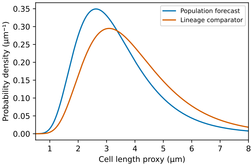
LB: predicted profiles
