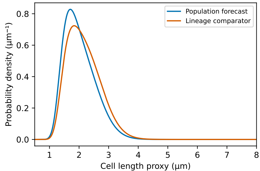
M9-succinate: predicted profiles
