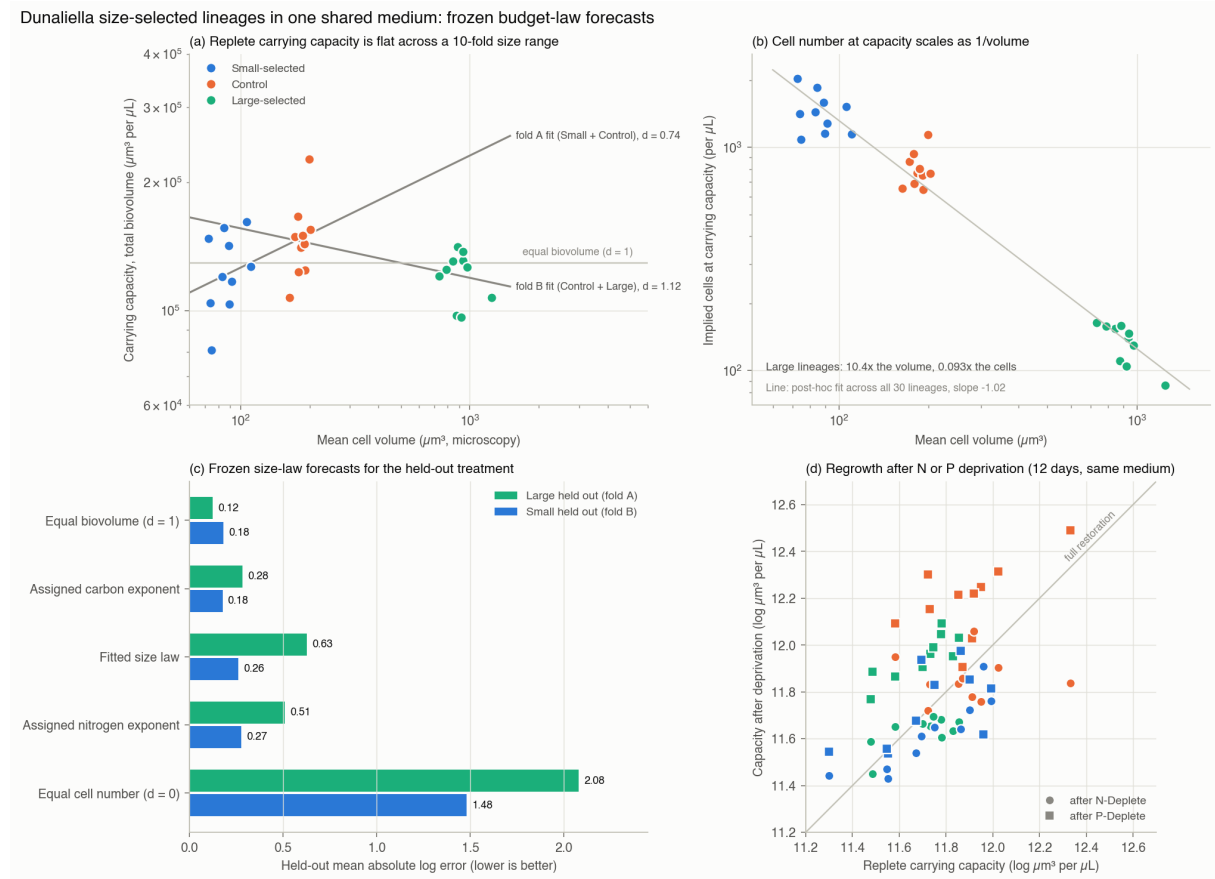
Figure 2. Size-selected Dunaliella lineages regrown in one shared medium, from the data of Malerba et al. (2018). (a) Replete carrying capacity in total biovolume against mean cell volume, with the two cross-fitted size laws and the equal-biovolume law. (b) Implied cell number at capacity. (c) Held-out errors of the frozen forecasts. (d) Capacity after N or P deprivation against replete capacity. Generated from retained outputs by report_dunaliella_size_budget.py .
