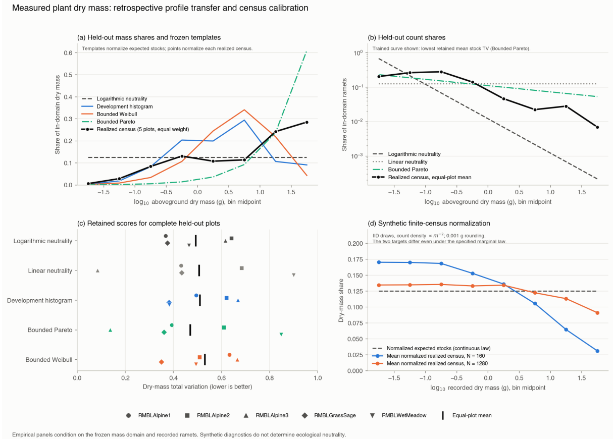
Figure 3. Directly weighed plant profiles and synthetic observation limits. (a) Equal-plot mean Colorado biomass shares and transferred stock templates. (b) Count shares and retained count forecasts. (c) Each plot’s biomass discrepancy and the five means. (d) Mean normalized census shares under iid logarithmic neutrality, compared with normalized expected stocks. All panels read retained outputs; report_plant_biomass_profile.py performs presentation only. Prior raw exposure and excluded biomass are retained.
