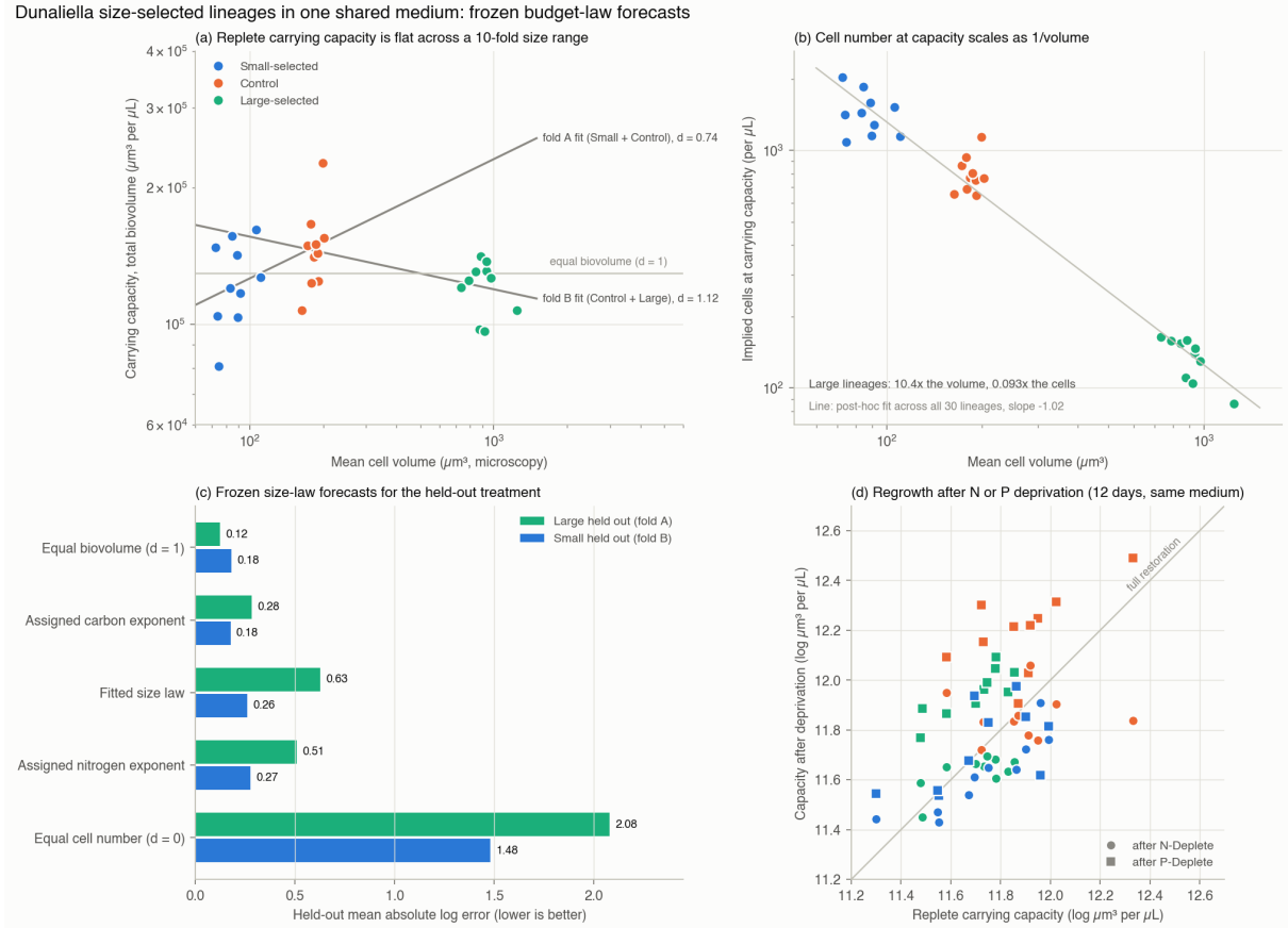
Figure 2. Size-selected Dunaliella lineages regrown in one shared medium, from the data of Malerba et al. (2018). (a) Replete carrying capacity in total biovolume against mean cell volume, with the two cross-fitted size laws and the equal-biovolume law. (b) Implied cell number at capacity. (c) Held-out errors of the frozen forecasts. (d) Capacity after N or P deprivation against replete capacity. Generated from retained outputs by report_dunaliella_size_budget.py .
