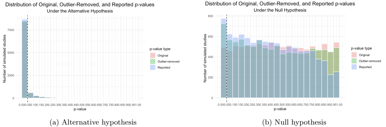
Figure 9: Distribution of the original, outlier-removed, and reported p-values under the alternative and null hypotheses (QRP1).
