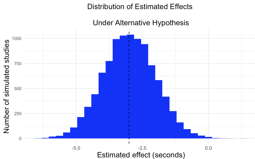
Figure 6: Distribution of estimated effects across simulated studies under the alternative hypothesis.
