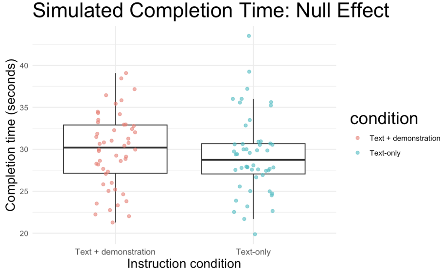
Figure 2: Boxplots of the distribution of simulated completion time under null dataset.
