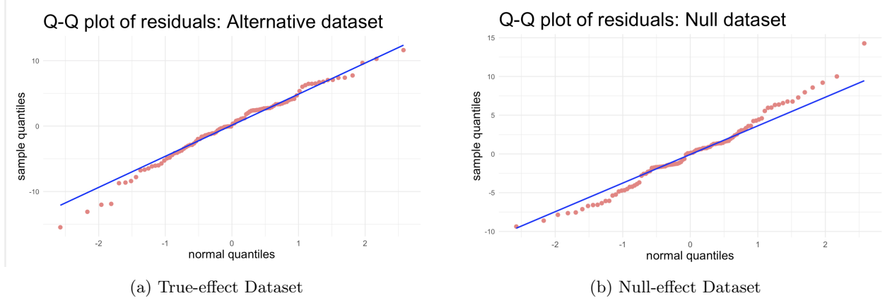
Figure 3: Q-Q plots of residuals under alternative and null dataset.
