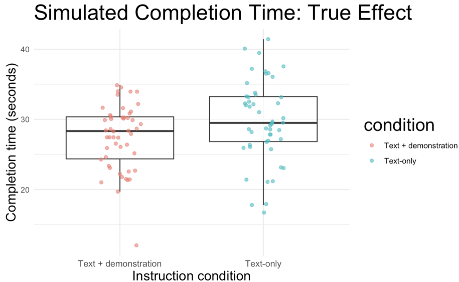
Figure 1: Boxplots of the distribution of simulated completion time under true-effect dataset.
