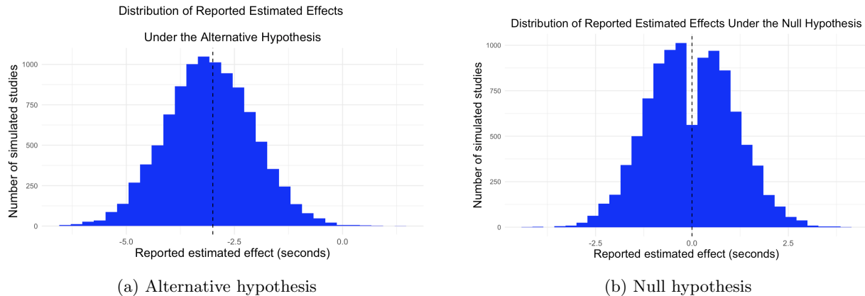
Figure 10: Distribution of selectively reported estimated effects under the alternative and null hypotheses (QRP1).
