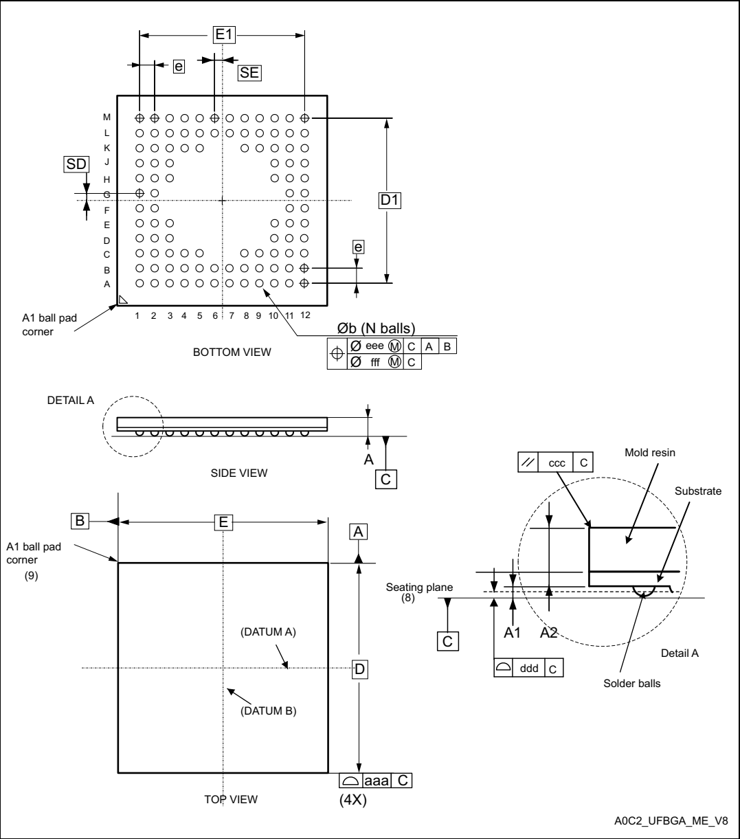
Figure 49. UFBGA100 - Outline (13)
