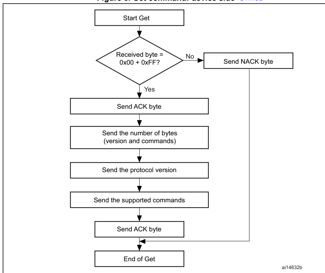
Figure 3. Get command: device side STM32
