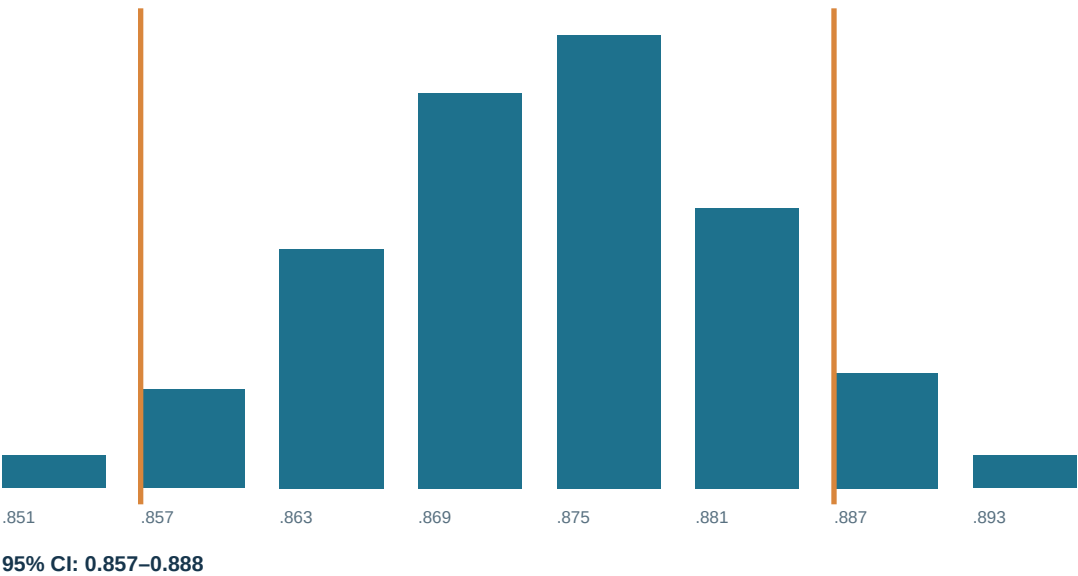
bootstrap resamples (n=200)
