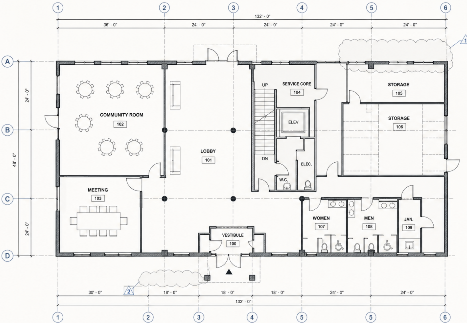
1 GROUND FLOOR PLAN 1/8" = 1'-0"
