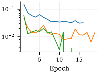
MMD 2 penalty
