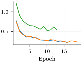
Classification loss
