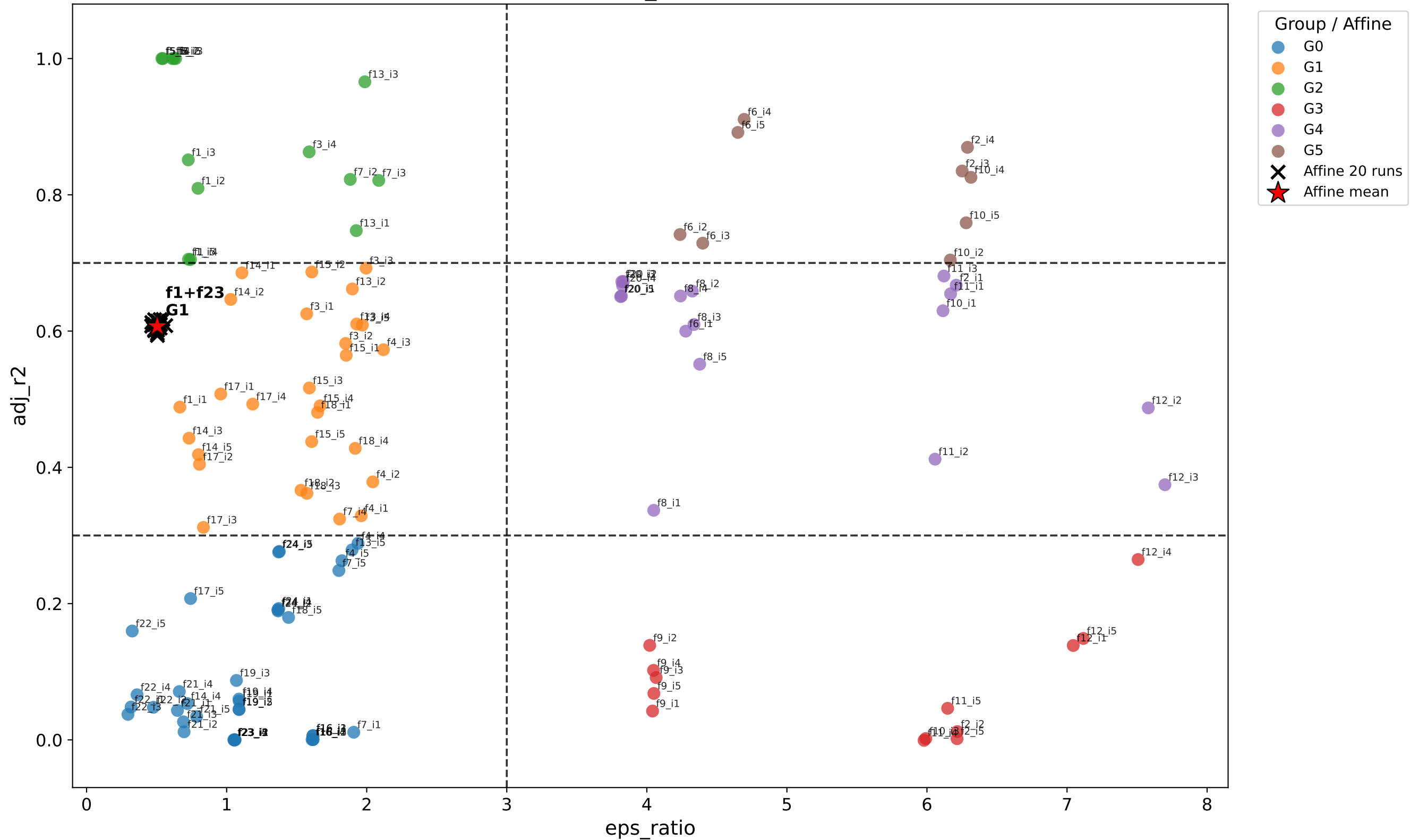
Affine function f1_f23 assigned to ELA grouping 0307_main
