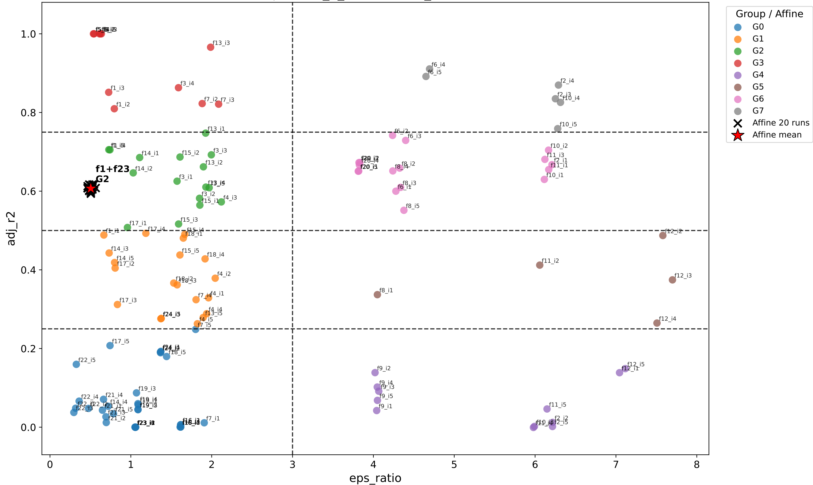
Affine function f1_f23 assigned to ELA grouping eps2bins_4_r025050075_instance
