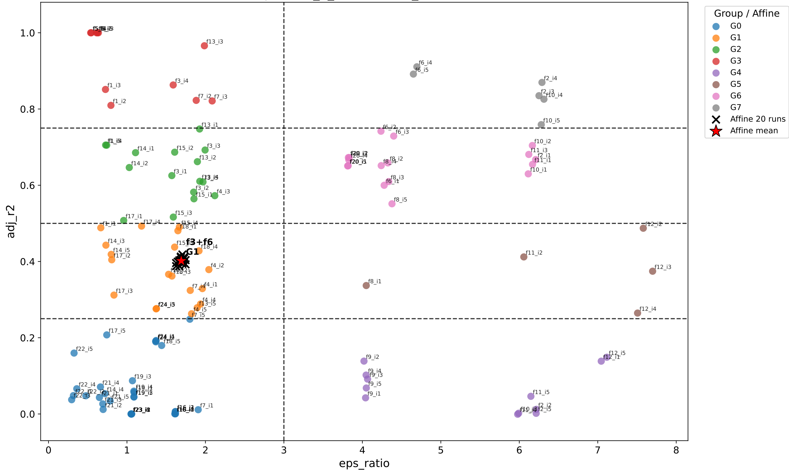
Affine function f3_f6 assigned to ELA grouping eps2bins_4_r025050075_instance
