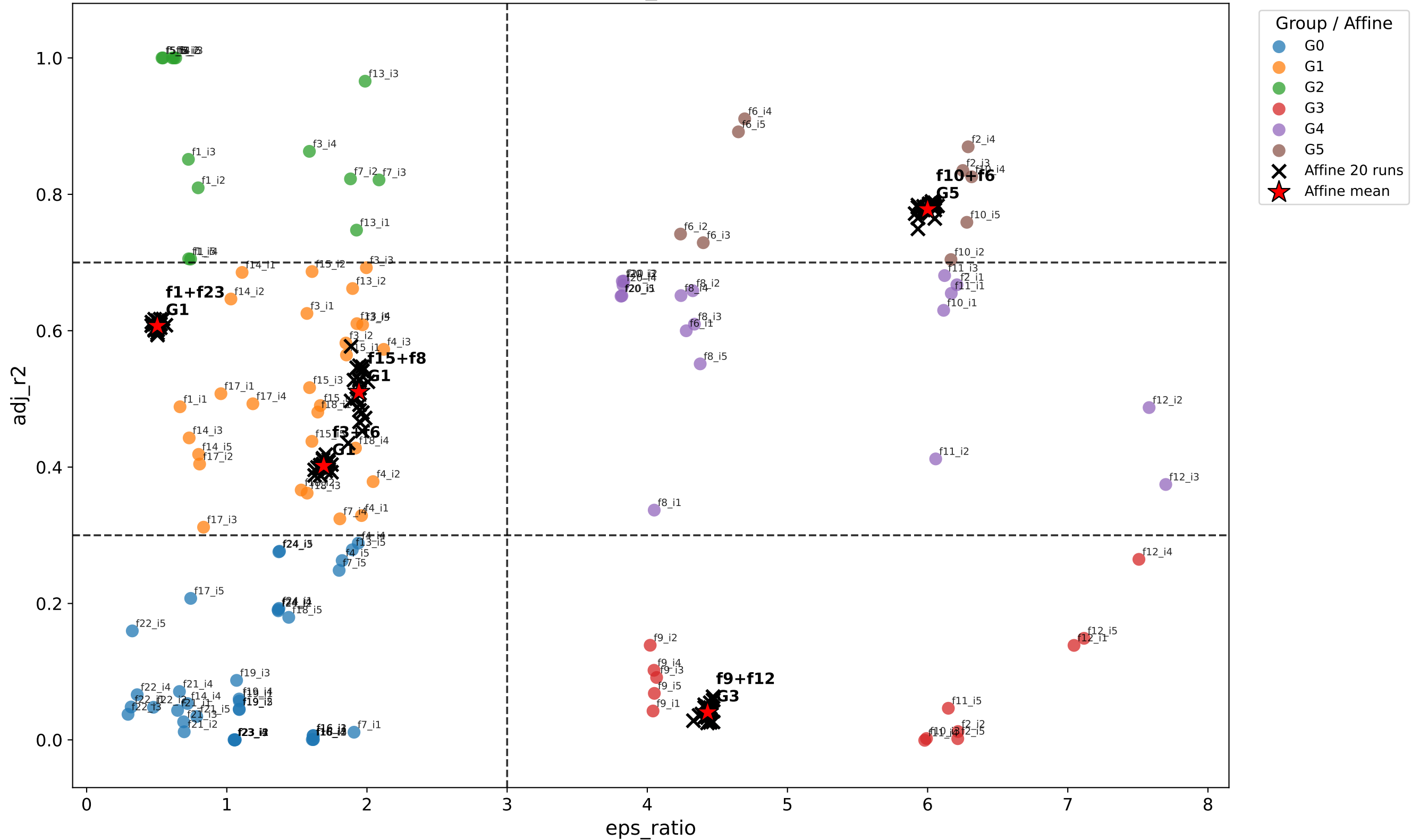
Affine BBOB functions assigned to ELA grouping 0307_main
