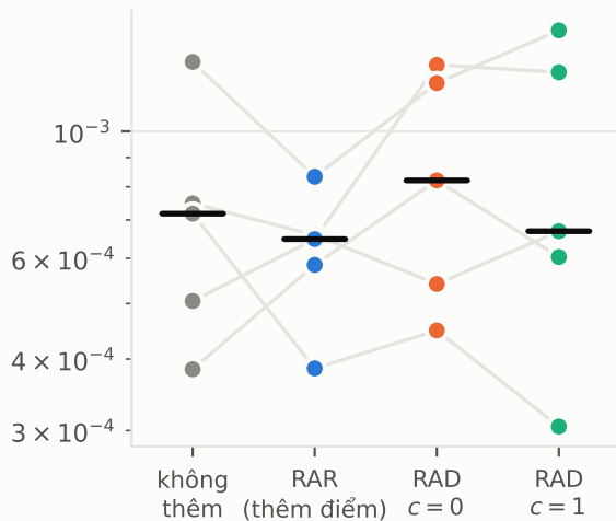
(a) \varepsilon_{L^2}
