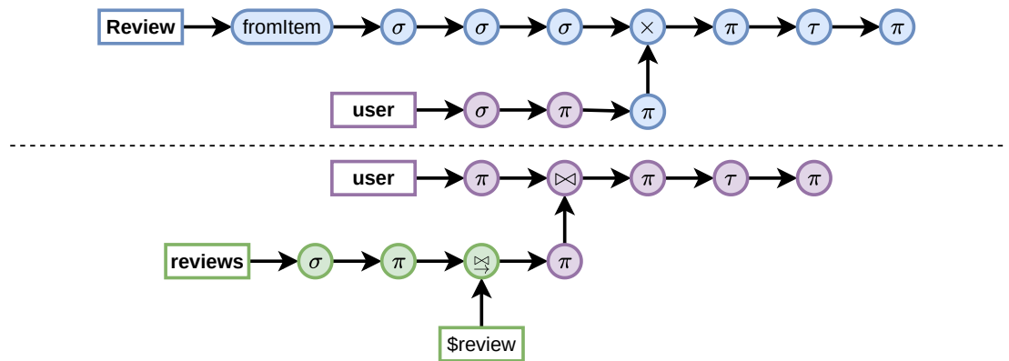
Figure 0.16 Unified algebra representation of the queries from Example 0.13. The colors correspond to the original languages— SQL (purple), Cypher (blue), and XQuery (green). Some operations (e.g., calculations, tree joins) were omitted for clarity.
