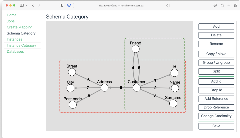
Figure 2.5 A screenshot of MM-evocat
