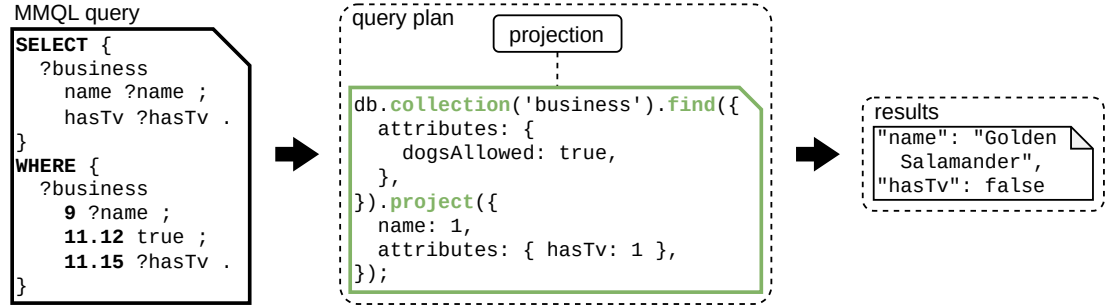
Figure 0.5 A MMQL query from Example 0.5 and its translation to the MongoDB query language [26].
