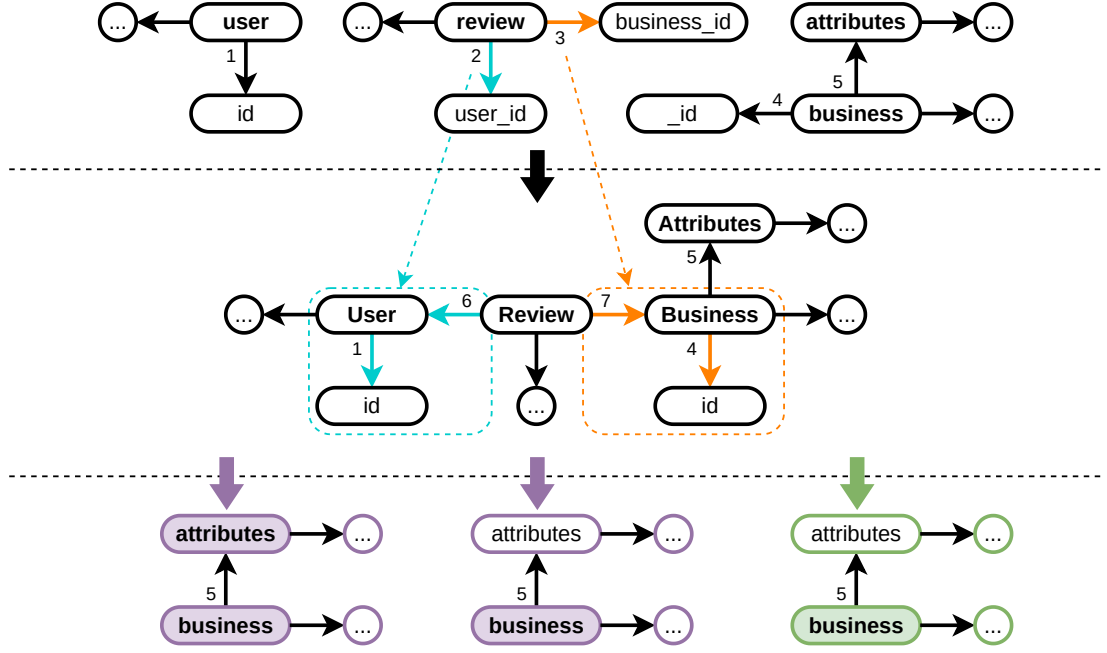
Figure 0.15 Benchmark creation steps from Example 0.12: inferred conceptual schema, refined conceptual schema, and three alternative logical representations.
