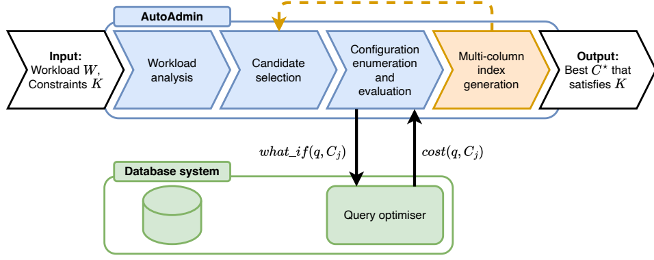
Figure 6.5 AutoAdmin architecture
