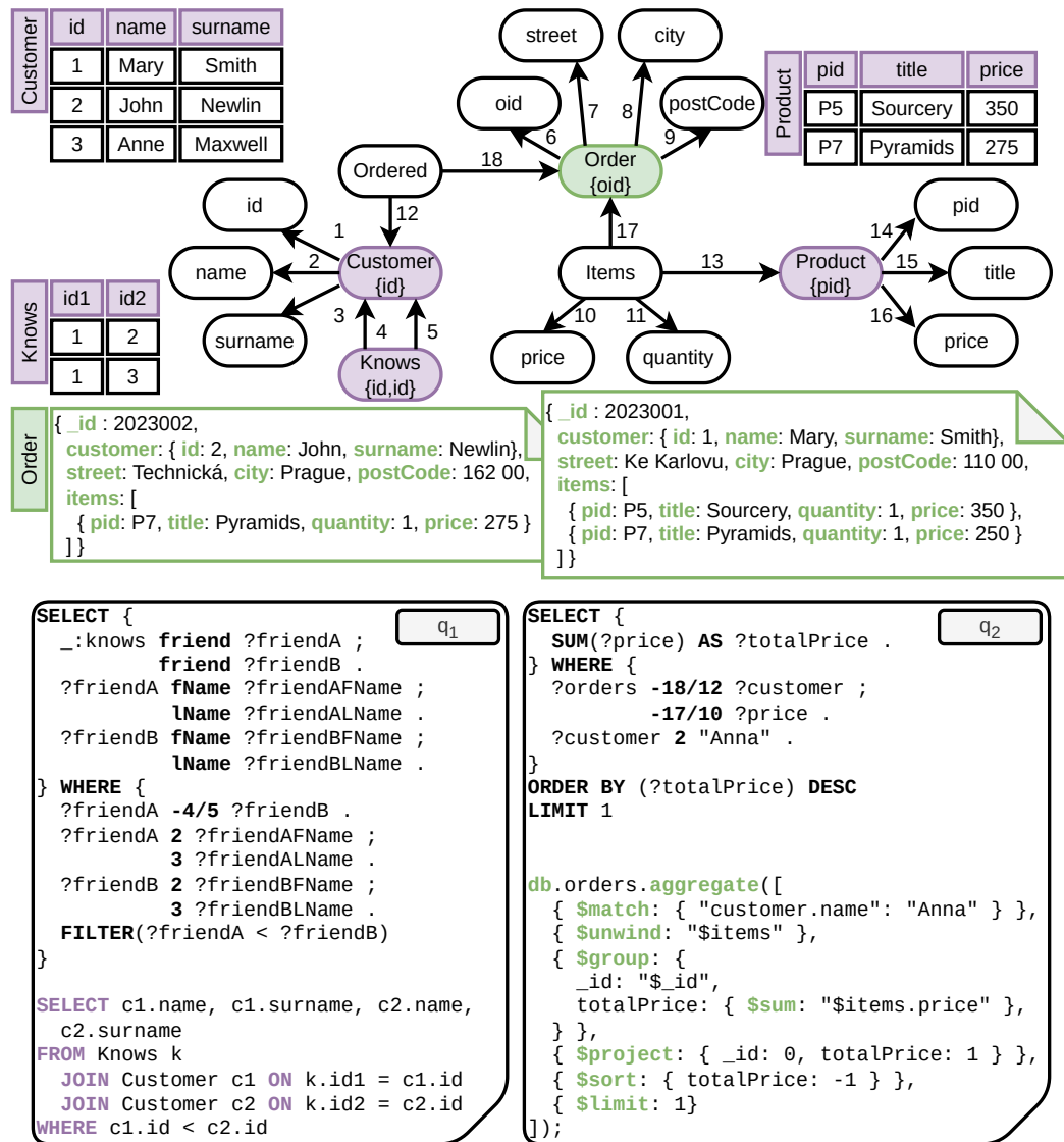
Figure 3.5 Version 3B – a multi-model mapping (PostgreSQL and MongoDB)
