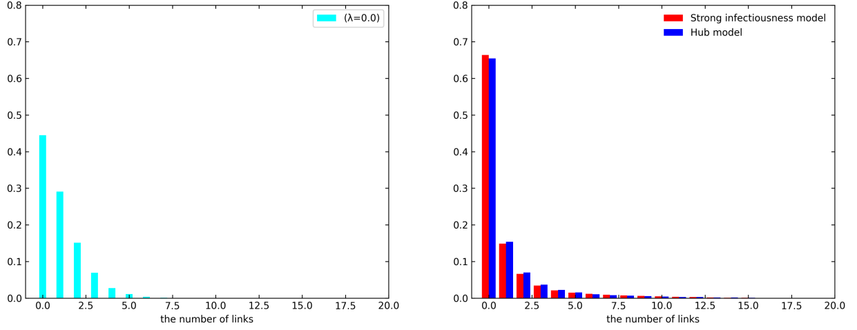
Figure 4: Reimplemented secondary infection distributions at \rho\pi r_0^2 = 15
