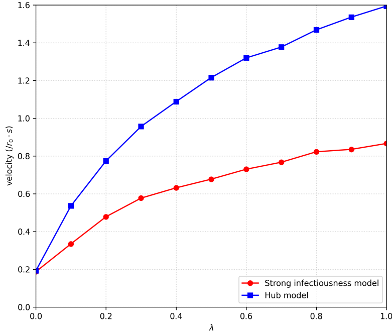
Figure 6: Reimplemented propagation-speed comparison between the strong infectiousness and hub models at \rho\pi r_0^2 = 20
