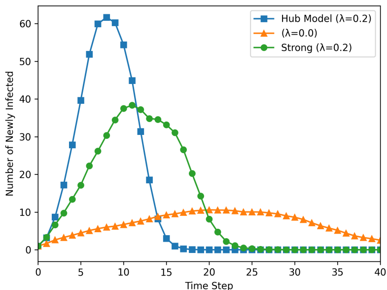
Figure 3: Reimplemented epidemic curves at \rho\pi r_0^2 = 20
