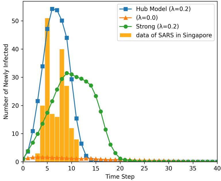
Figure 5: Reimplemented comparison between the simulated epidemic curves and the Singapore SARS epidemic curve
