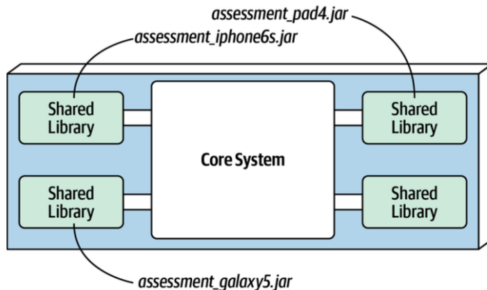
Shared library plug-in implementation
