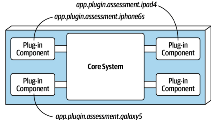
Package or namespace plug-in implementation
