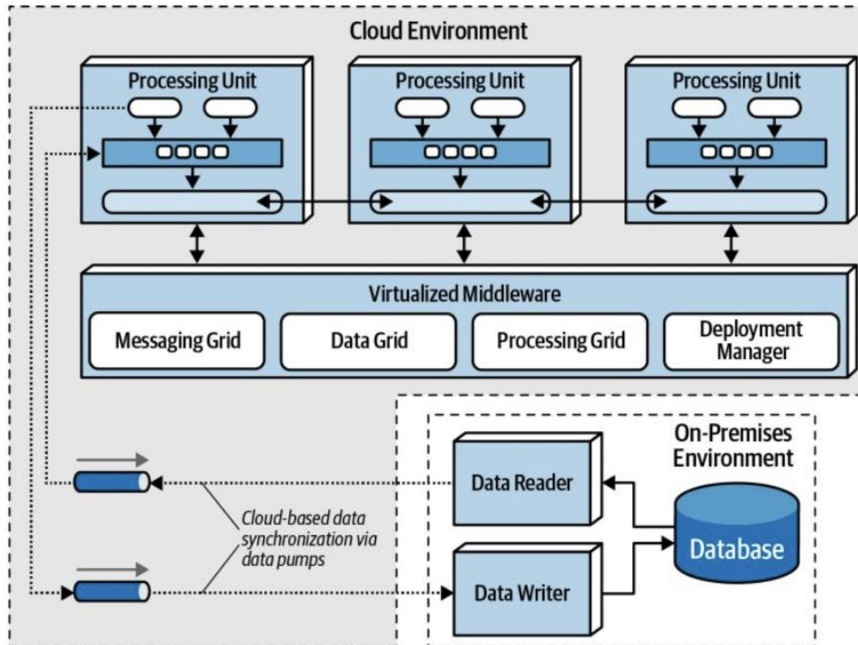
Hybrid cloud-based and on-prem topology
