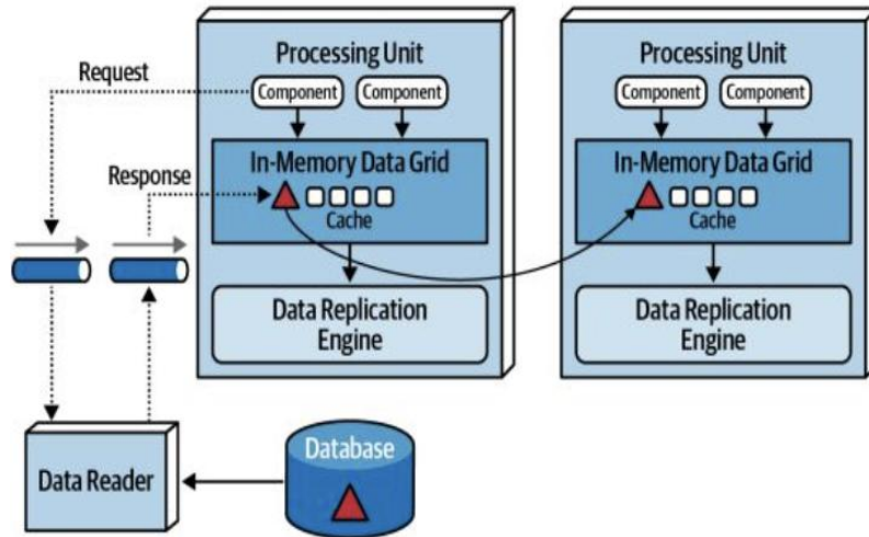
Data reader with reverse data pump
