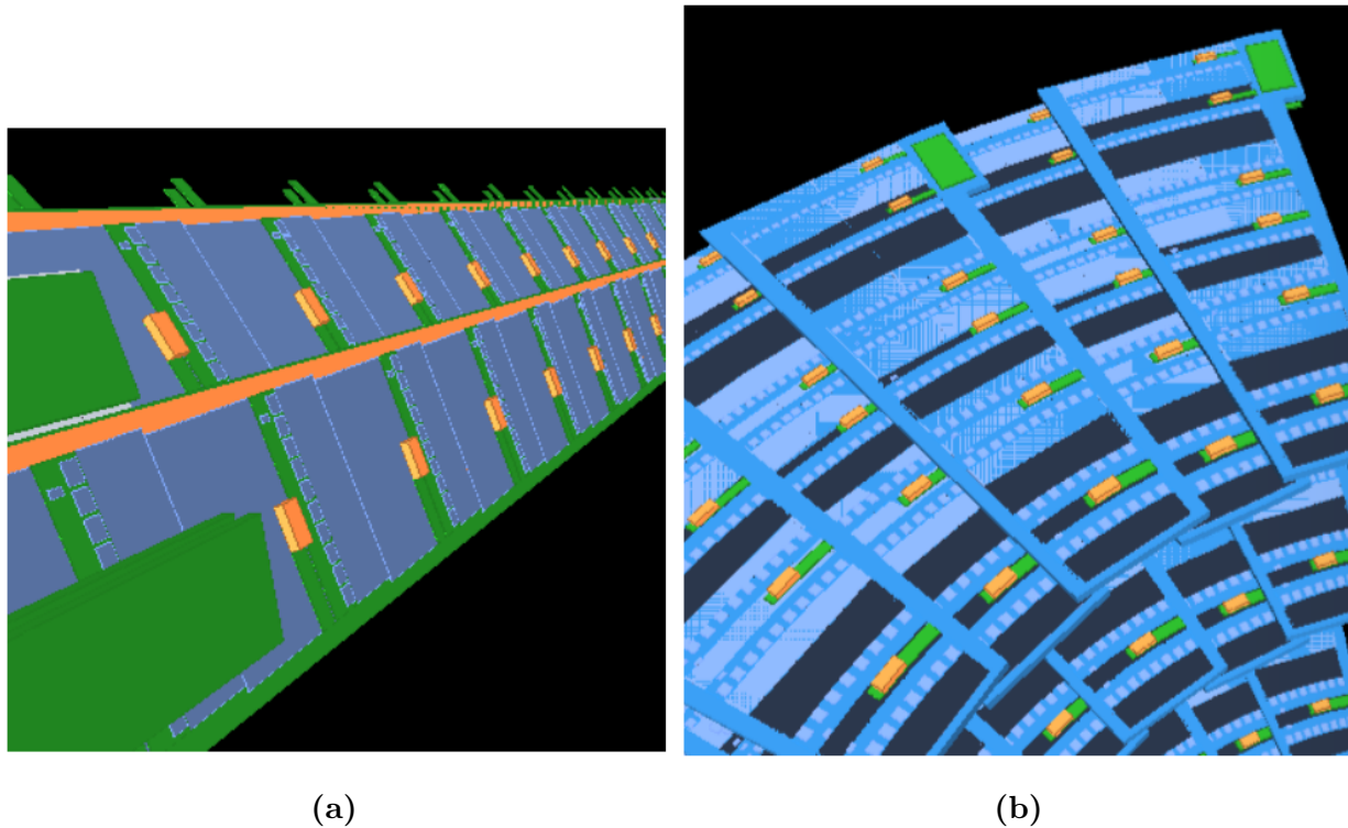
Figure 6.5: Displays of the GEANT4 geometry model of the strip barrel staves (left) and the endcap petals (right). Figure taken from reference [109].
