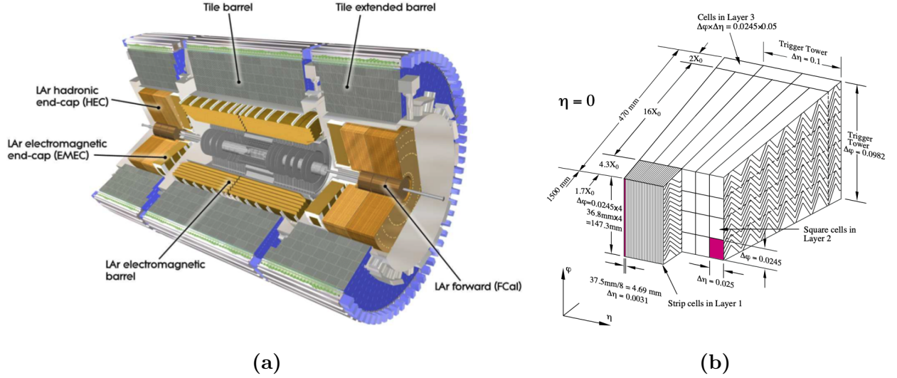
Figure 3.4: (a) Layout of the ATLAS calorimetry system, and (b) sketch of a barrel module of the electromagnetic calorimeter [38].
