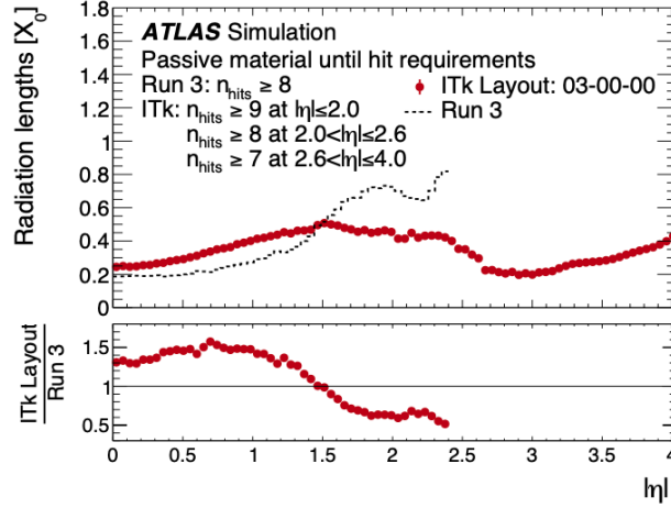
(c) Radiation length to reach reconstructible number of hits [107]
