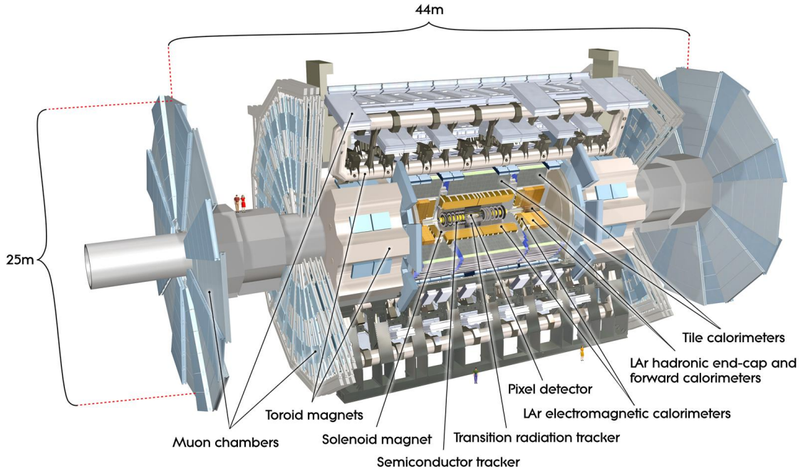
Figure 3.1: The ATLAS detectors and its components [31]
