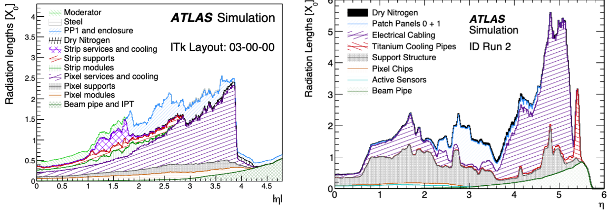
(a) ITk radiation length [107]
