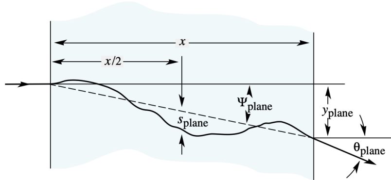
Figure 6.9: Schematic of the calculation of macroscopic mean deflection angle caused by multiple scattering [22].
