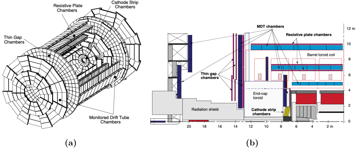
Figure 3.5: (a) Layout of the ATLAS Muon Spectrometer system, and (b) a sideview of one quadrant of the MS [39].
