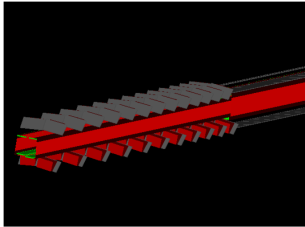
Figure 6.4: An illustration of the GEANT4 geometry model of the outer barrel longeron stave with mounted inclined and flat modules. Figure taken from reference [109].
