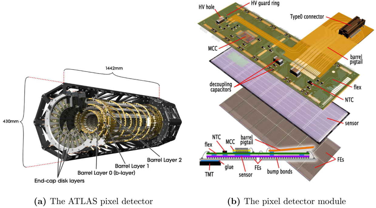
Figure 3.2: The ATLAS pixel detector and detector module. Figures taken from reference [33]
