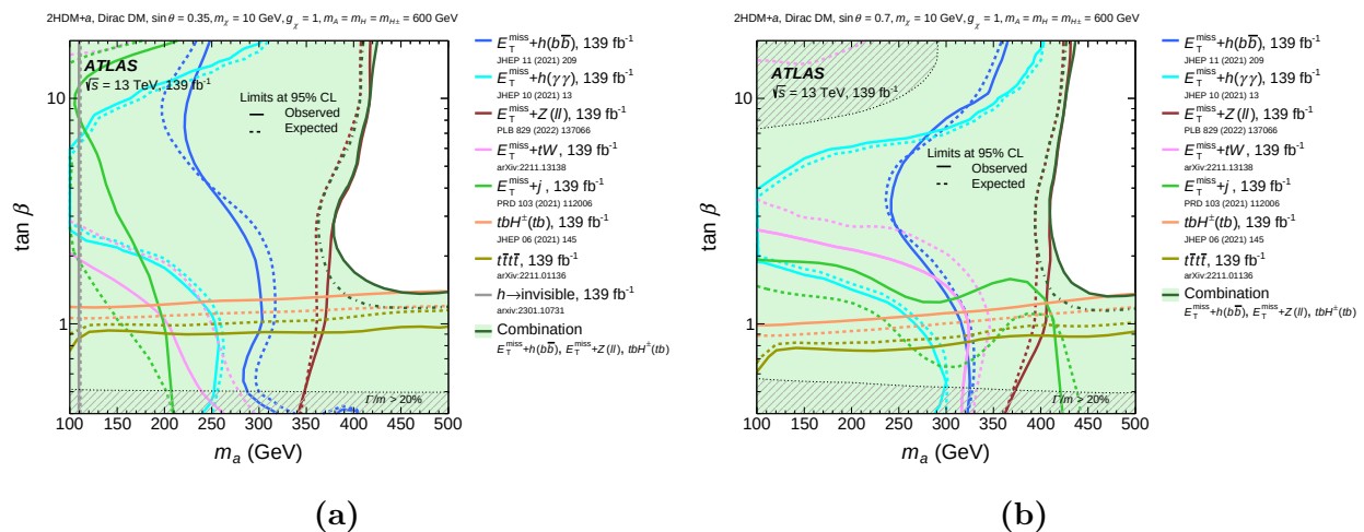
Figure 4.10: Observed and expected exclusion regions at 95% CL over the (m_a, \tan\beta) plane evaluated at 2HDM+ a mixing angles \sin\theta = 0.35 (a), and \sin\theta = 0.7 (b). The statistical combined contours are shown along with those from individual searches. In both subfigures, a dashed grey region indicates the region where the width of any of the Higgs boson exceeds 20% of its mass [59].
