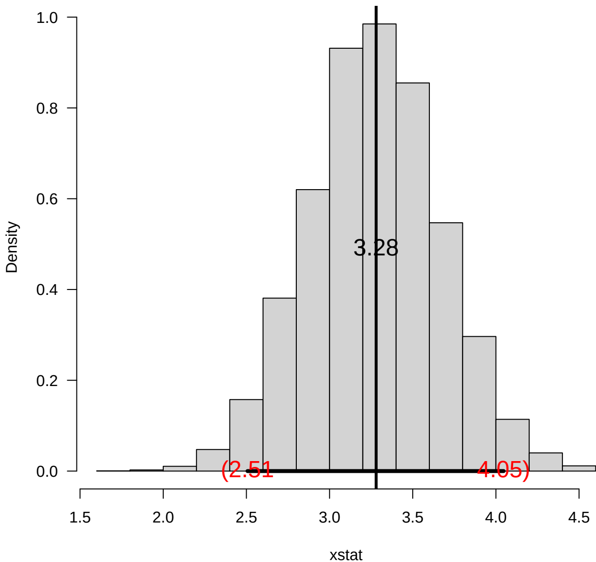
Histogram of Bootstrap sample statistics alpha=0.05 iter=10000
