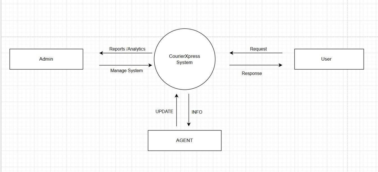
Figure 1: DFD level 0
