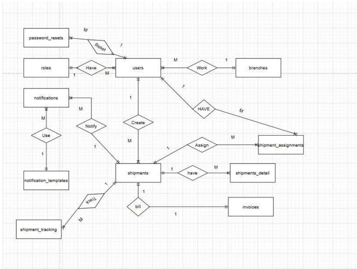
Figure 2: ERD Level 0
