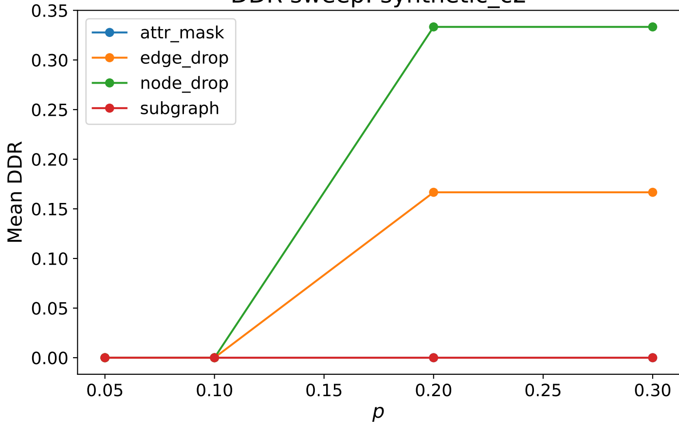
DDR sweep: synthetic_c2
