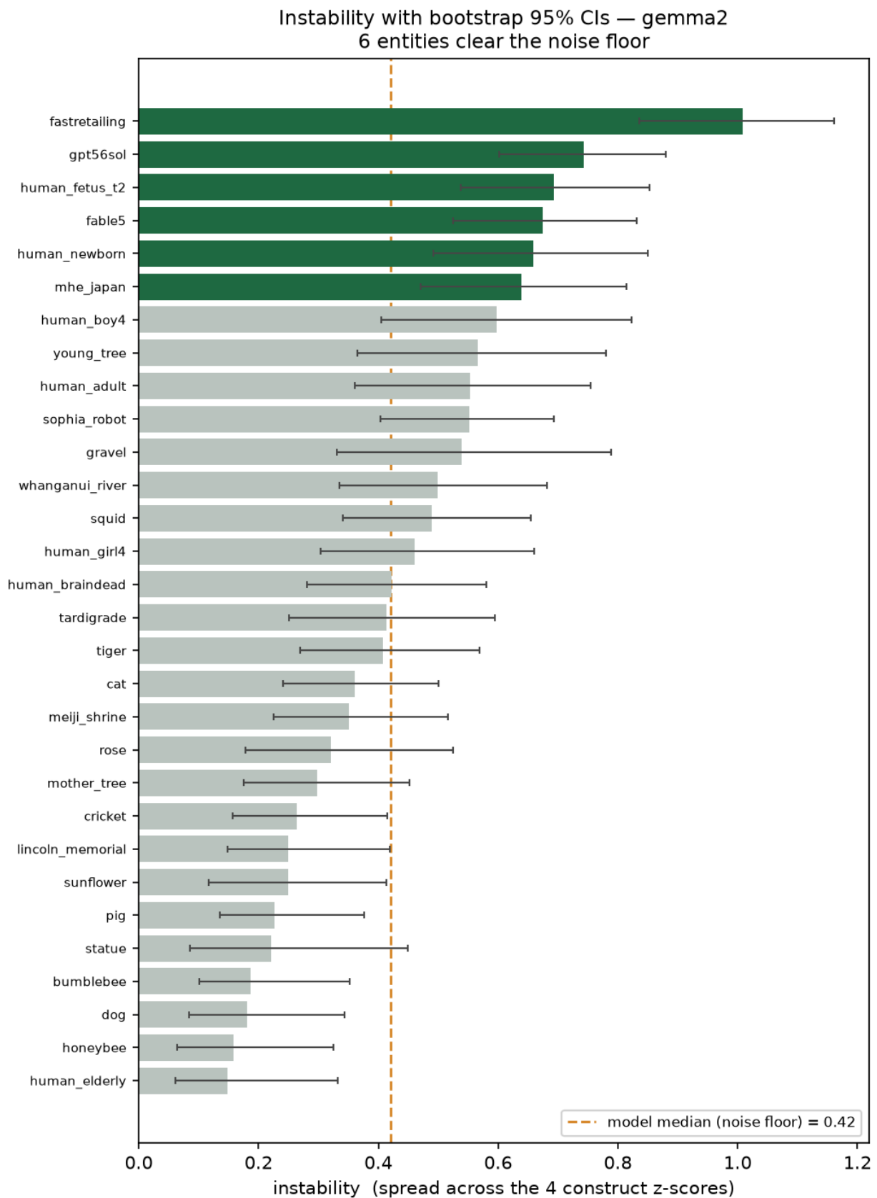
Figure A4. Instability with bootstrap confidence intervals vs the noise floor — Gemma 2 (all-8 bootstrap, bootstrap_ci_all18.csv; 6 of its 30 entities clear).
