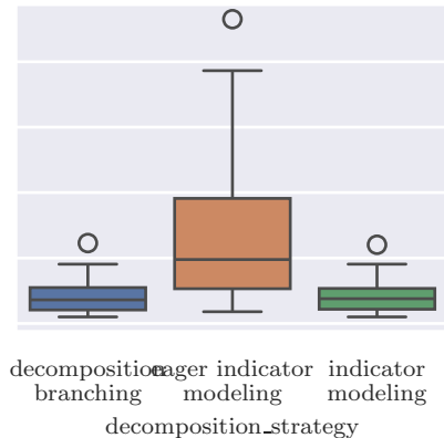
99 instances with gap
