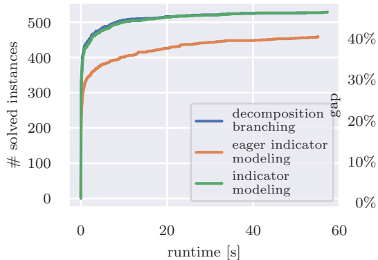
529 instances solved to optimality
