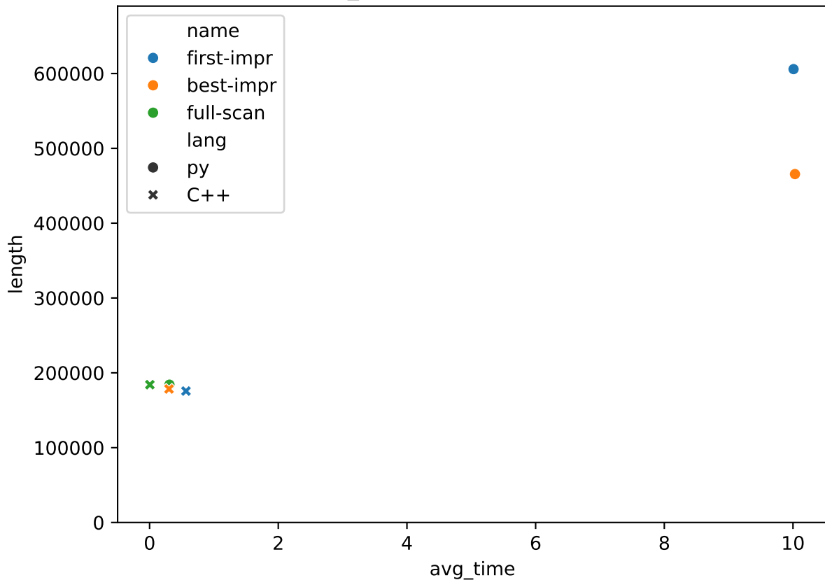
avg_time to length for n=500
