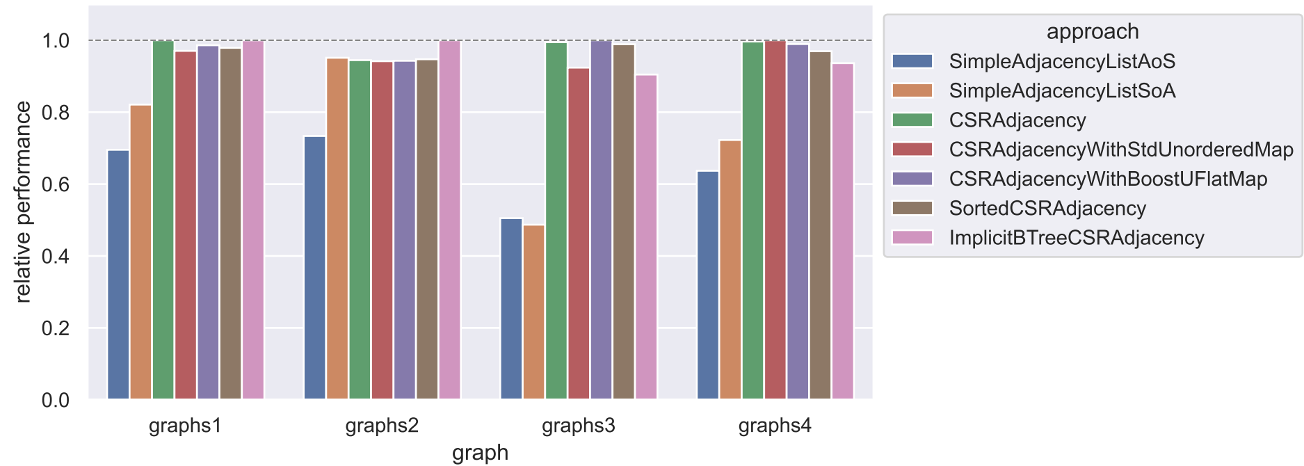
iterate_neighbors_random_vertex_order
