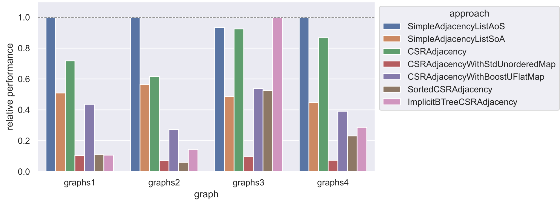
rebuild
