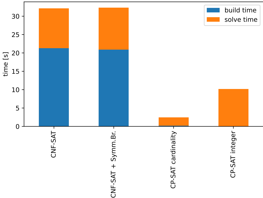
200 Queens benchmark
