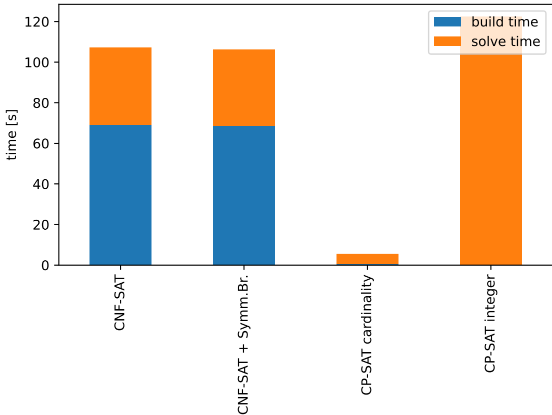
300 Queens benchmark
