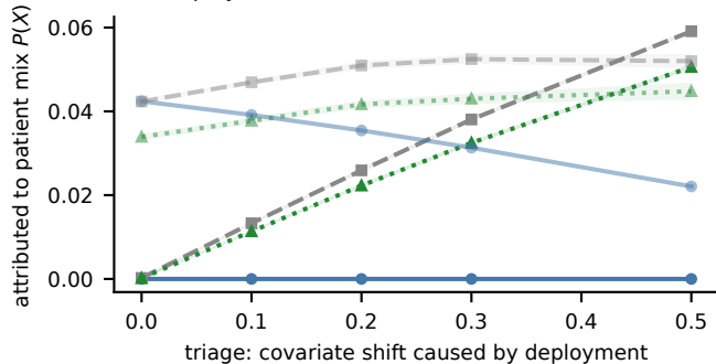
deployment-caused mix shift is booked to P(X)
