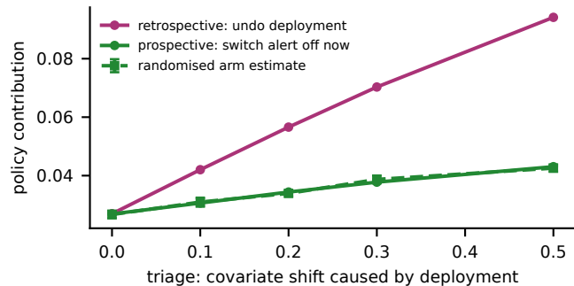
two policy estimands; randomisation recovers the decision one
