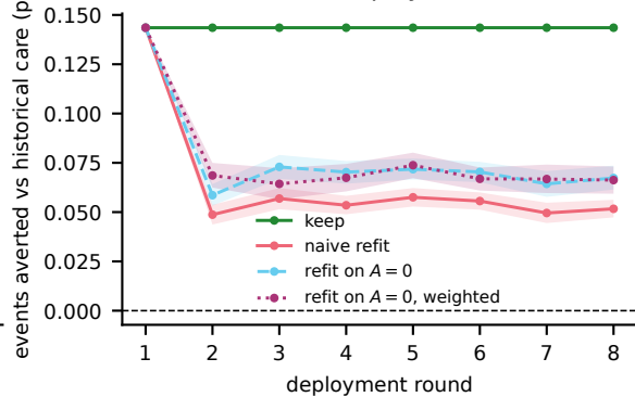
C: retrain and redeploy, fixed threshold
