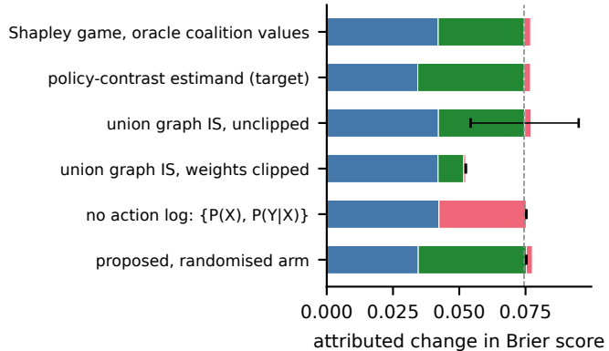
S4: covariate + outcome shift + deployment
