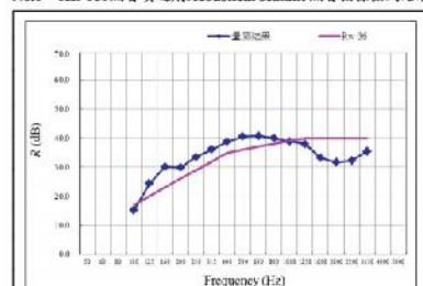
No.1：KL-101隔音填縫劑Acoustical sealant 隔音指標檢測結果
