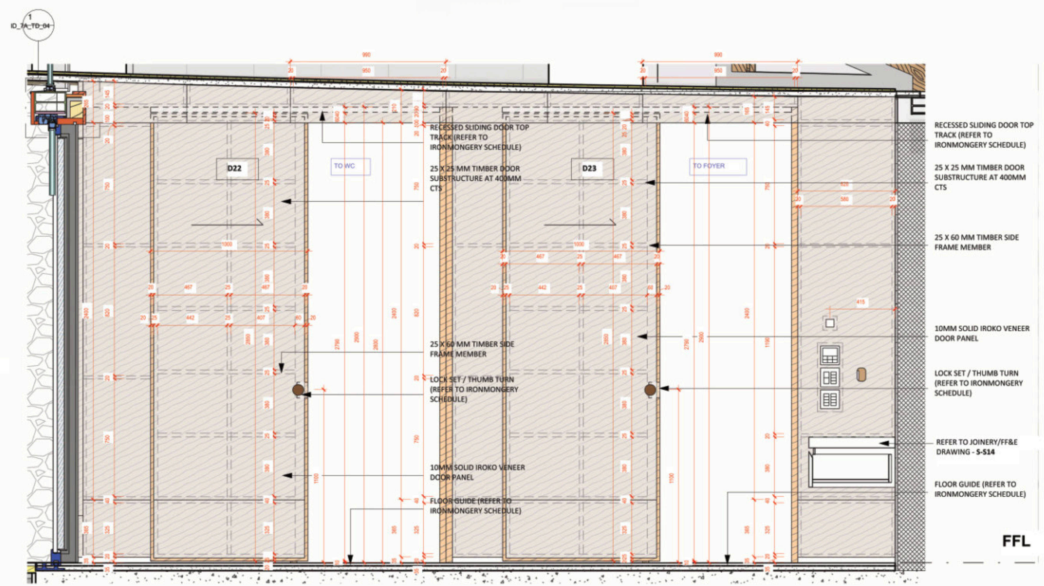
Front Elevation [with doors] NTS
