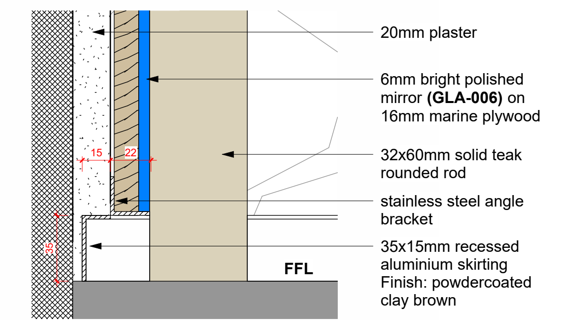
Callout - Skirting Detail | 1:2
