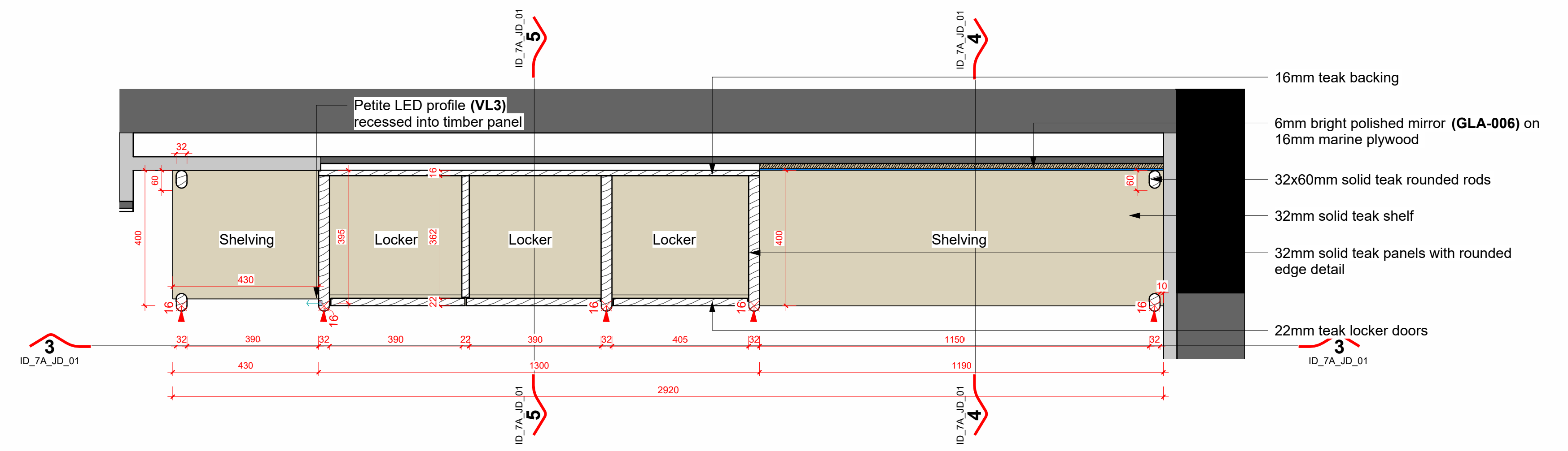
Floor Plan Lower View - Lockers | 1:10
