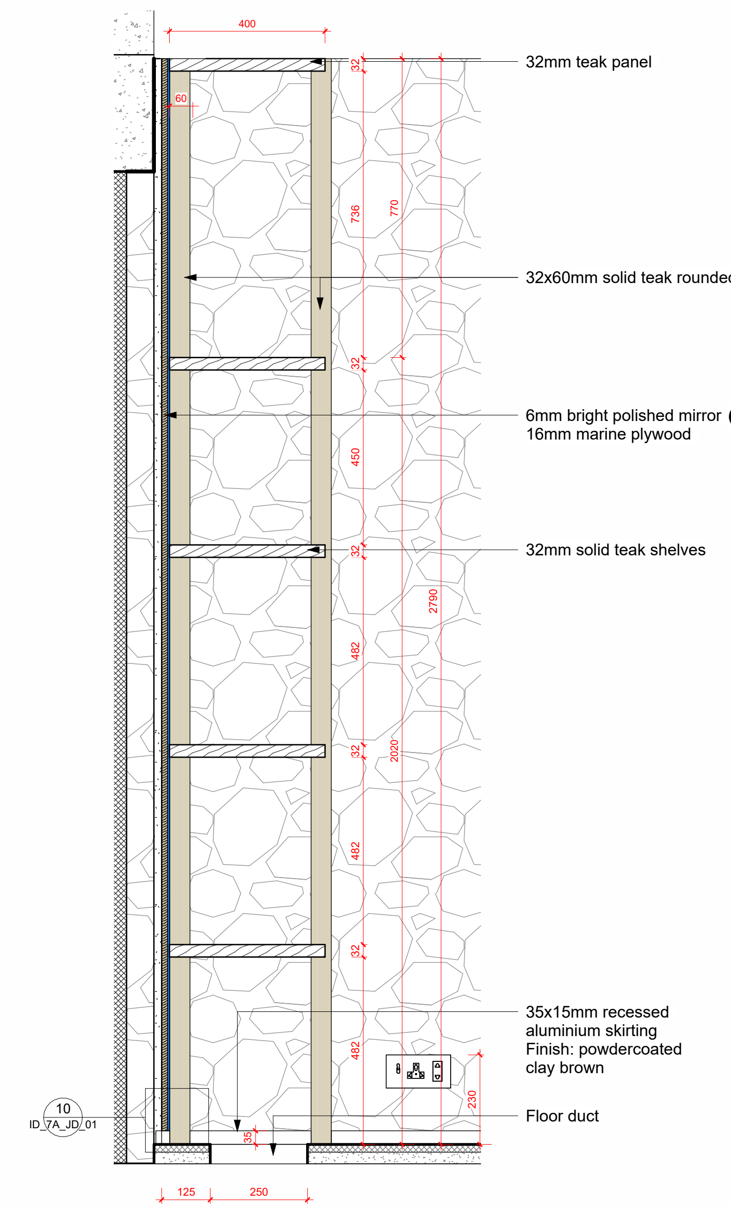
Section - Locker Shelves | 1:10
