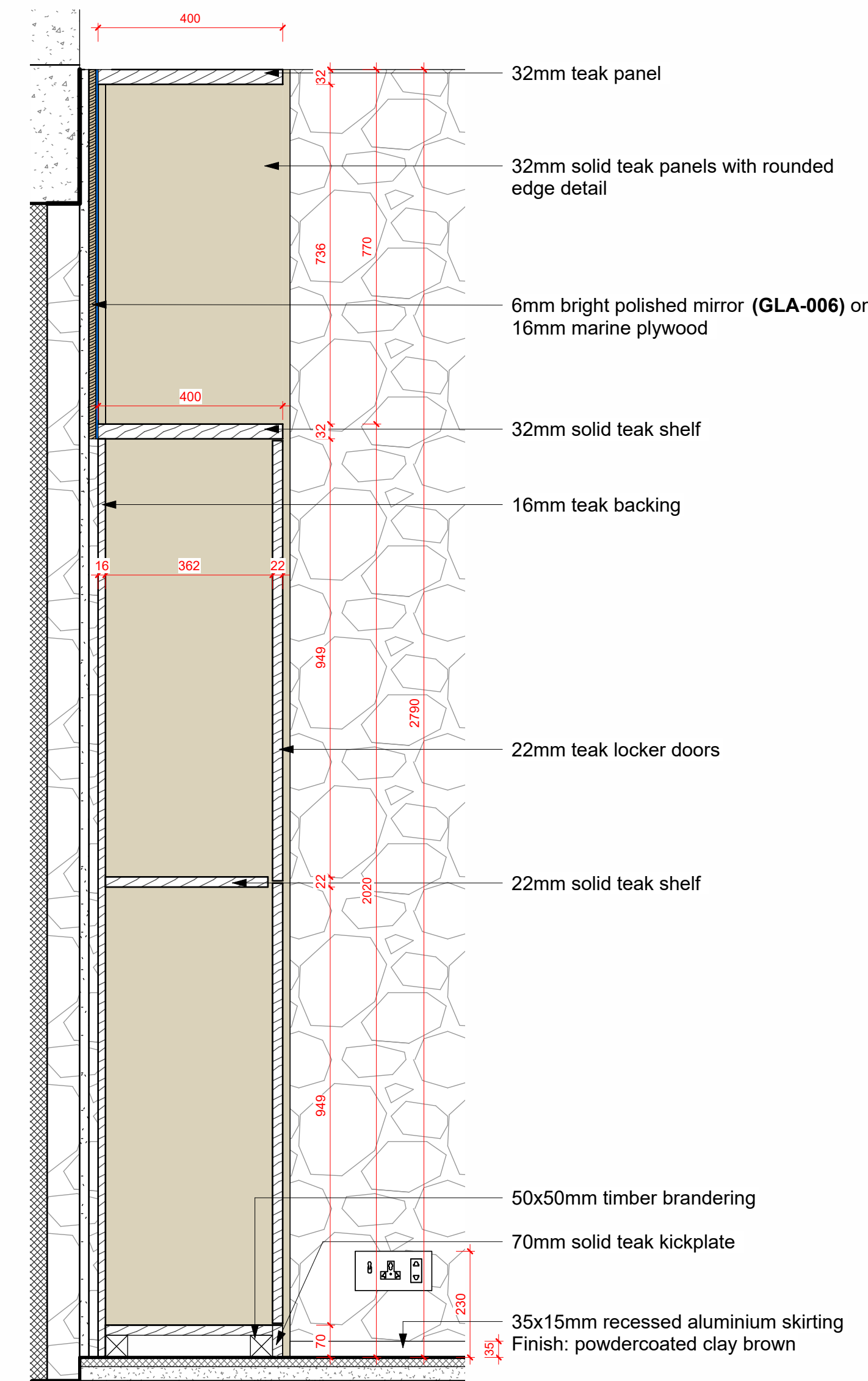
Section - Locker Cupboards | 1:10
