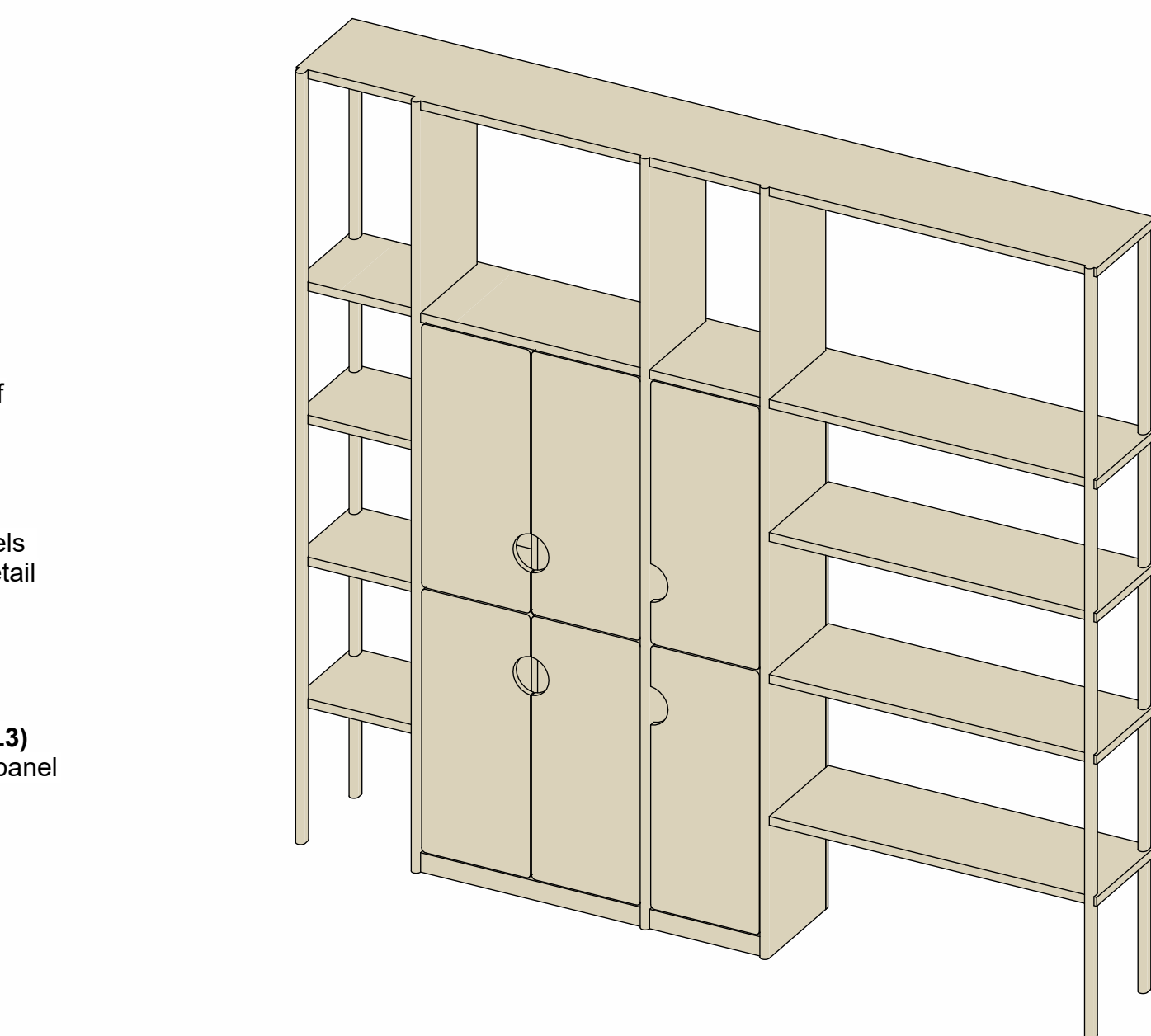
3D View - Lockers | 1:20
