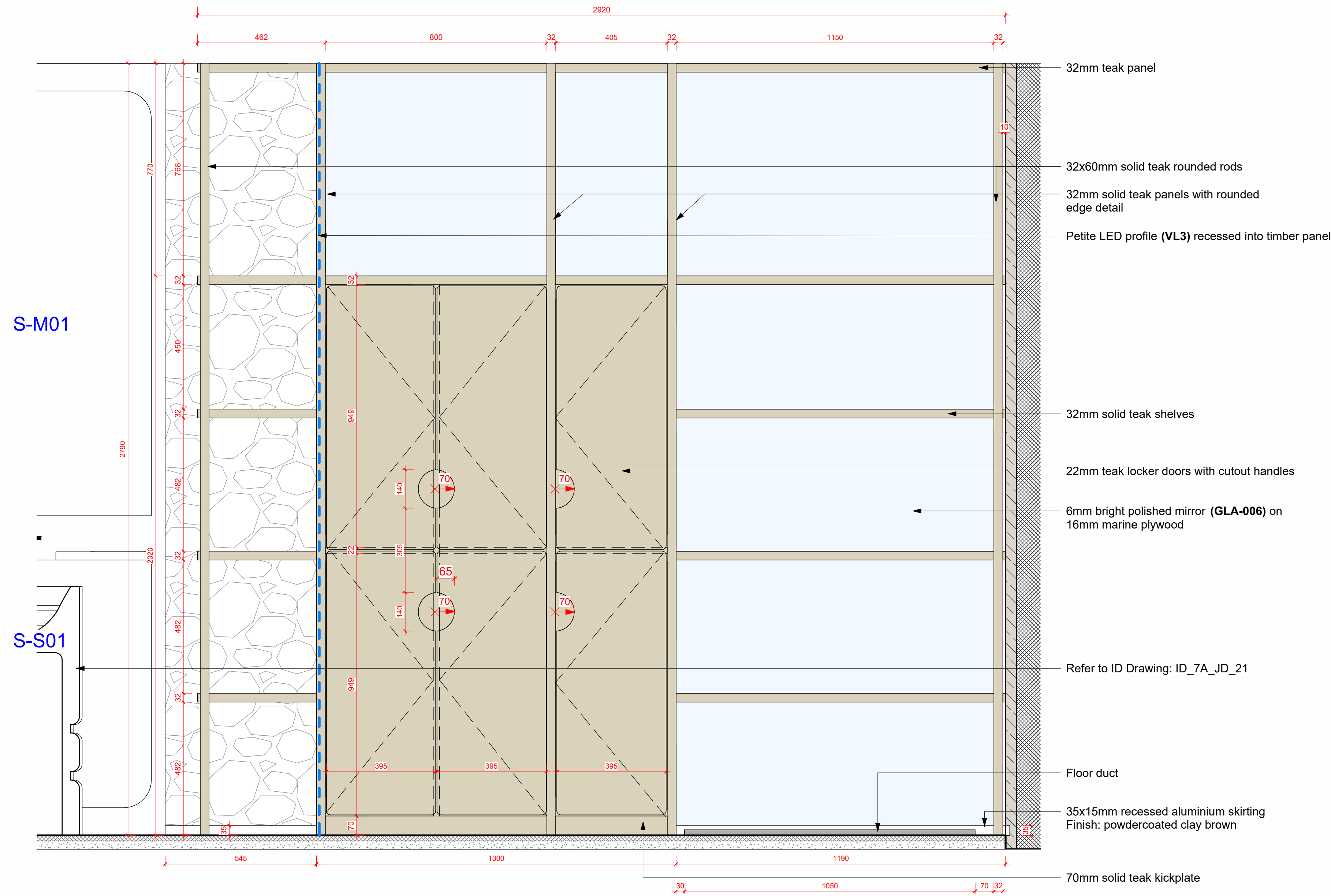
Front Elevation - Lockers | 1:10
